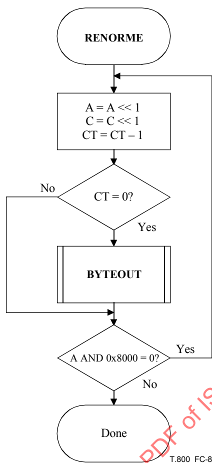
Figure C.8 – Encoder renormalization procedure
