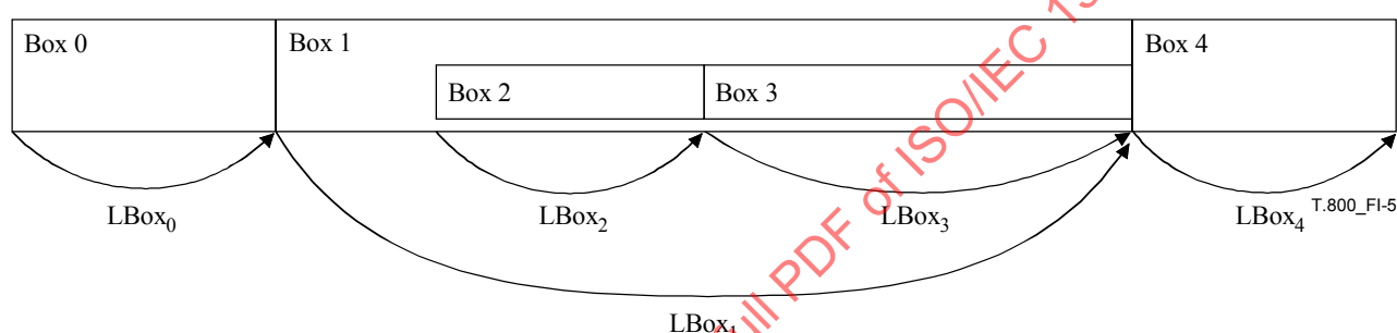
Figure I.5 – Illustration of box lengths
