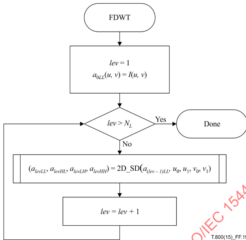
Figure F.19 – The FDWT procedure
