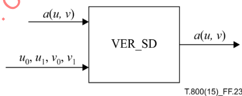
Figure F.23 – Inputs and outputs of the VER_SD procedure
