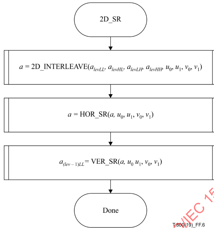
Figure F.6 – The 2D_SR procedure
