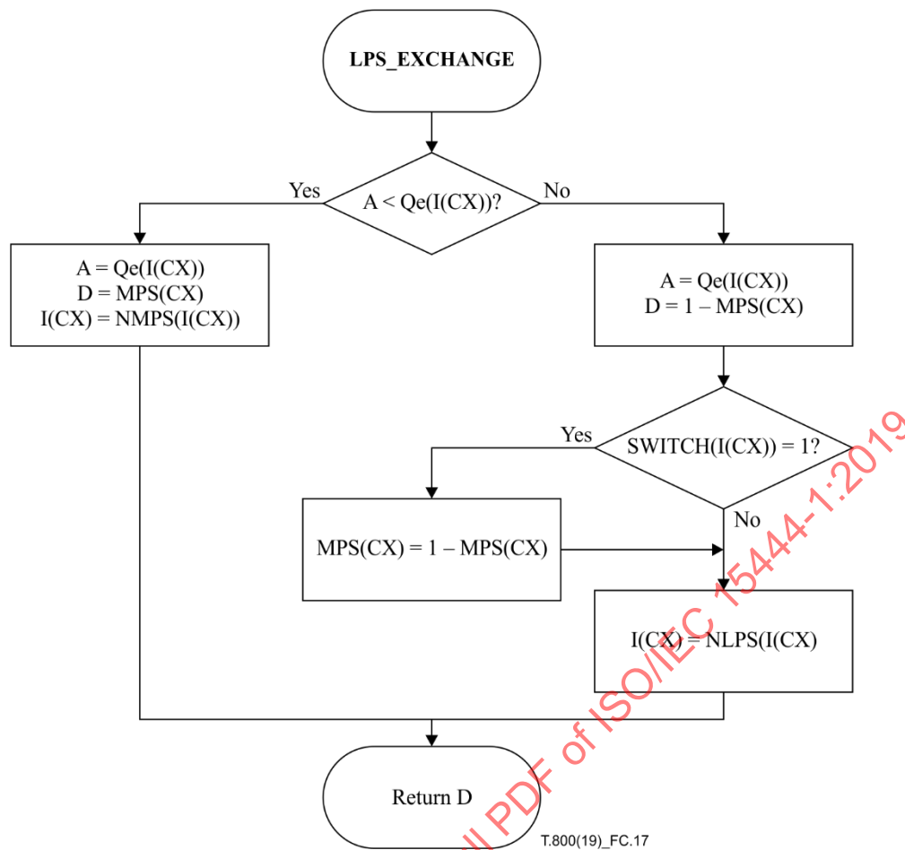
Figure C.17 – Decoder LPS path conditional exchange procedure
