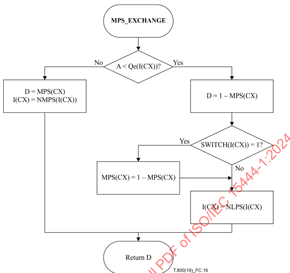
Figure C.16 – Decoder MPS path conditional exchange procedure
