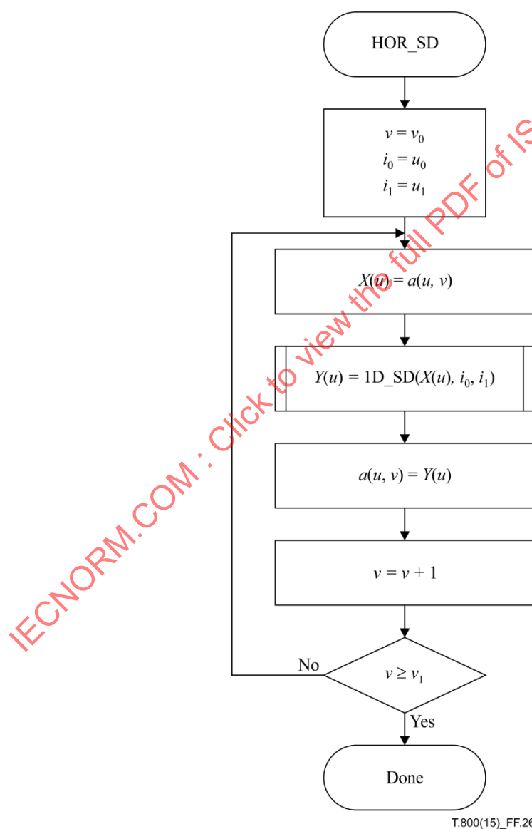
Figure F.26 – The HOR_SD procedure
