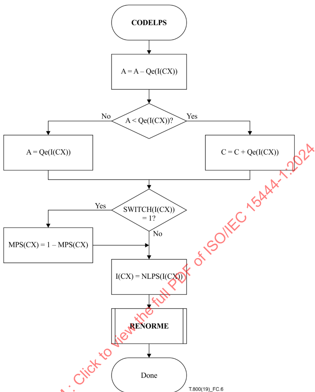
Figure C.6 – CODELPS procedure with conditional MPS/LPS exchange
