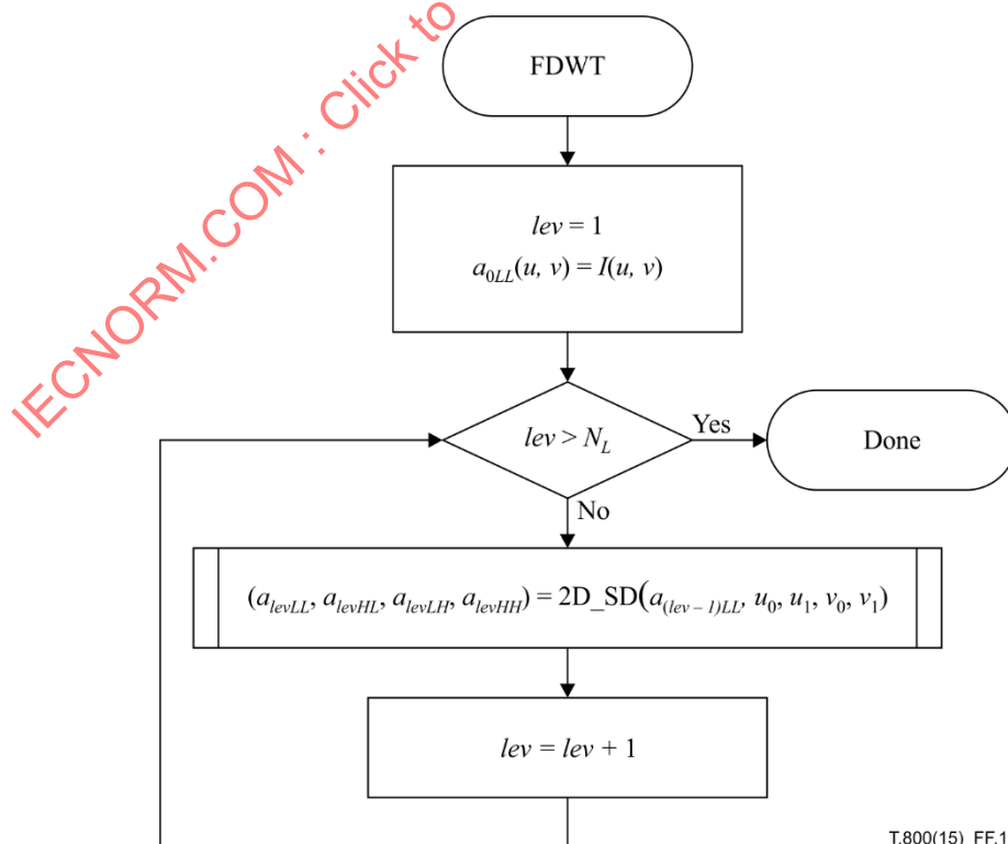
Figure F.19 – The FDWT procedure
