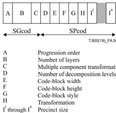
Figure A.9 – Coding style parameter diagram of the SGcod and SPcod parameters
