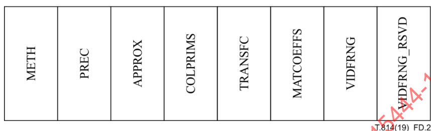
Figure D.2 – Organization of the contents of a Colour Specification box when METH = 5
