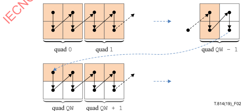
Figure 2 – Quad-based scanning pattern used in the HT cleanup pass
