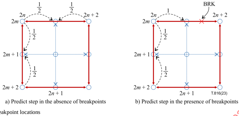
Figure 24 – Phase 2 predict step examples
