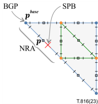
a) Example of a non-root arc with a spatially induced break at resolution r
