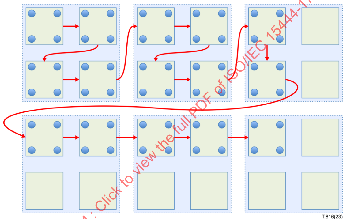
Figure 25 – Canonical scanning pattern used for the significance coding passes of CL band code-blocks in a QuadBPT component. In this case, missing cells within a 2 \times 2 group are not included in the scan
