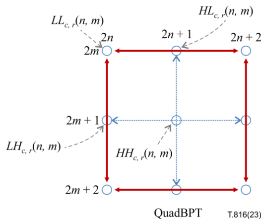
Figure 19 – Interleaving of sub-band coefficients to a quadrilateral grid for a given resolution r
