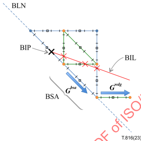
b) Horizontal root arc with binary flags ORN = Diagonal and DRCTNX\_FLAG_{induced} = 1 .
