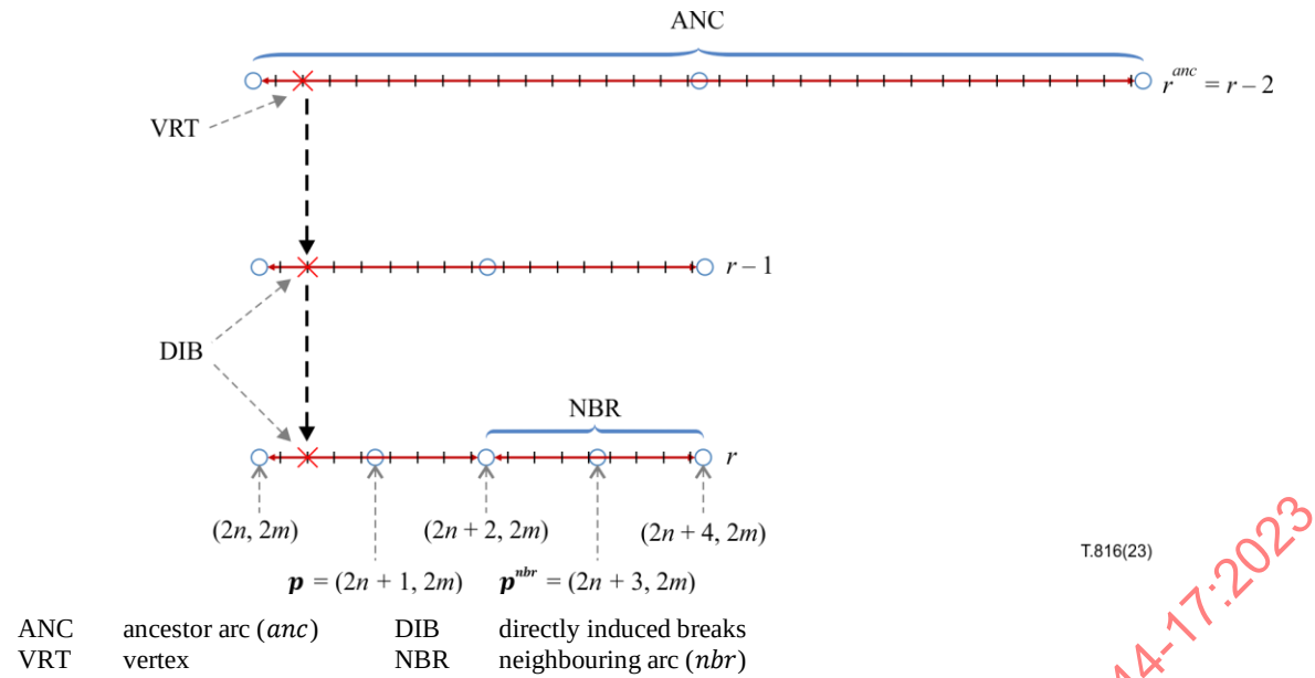
Figure 9 – Example of direct induction of a breakpoint
