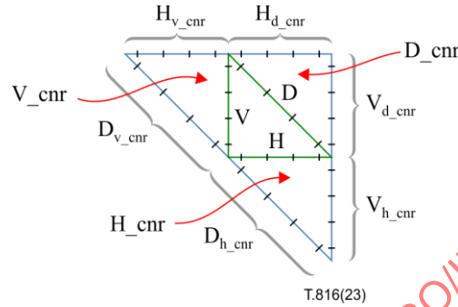
Figure 34 – Arc and corner labels for the TriBPT-LR arrangement
