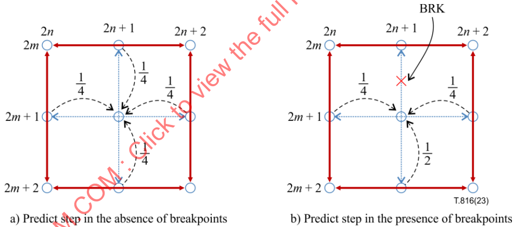
Figure 22 – Phase 1 predict step for (odd, odd) location (2n+1, 2m+1) with source locations of I_{c,r}^* shown
