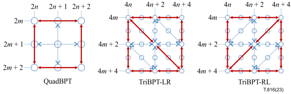
Figure 3 – Root arc (dotted lines) and non-root arcs (solid lines)
