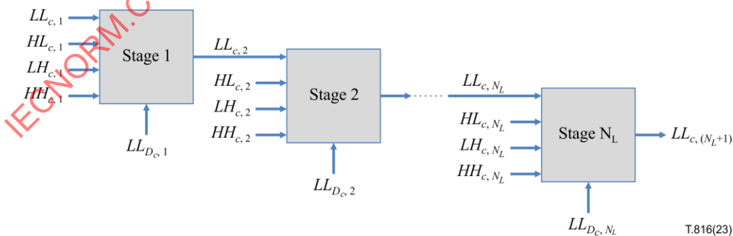
Figure 5 – Stages of the breakpoint dependent inverse discrete wavelet transform
