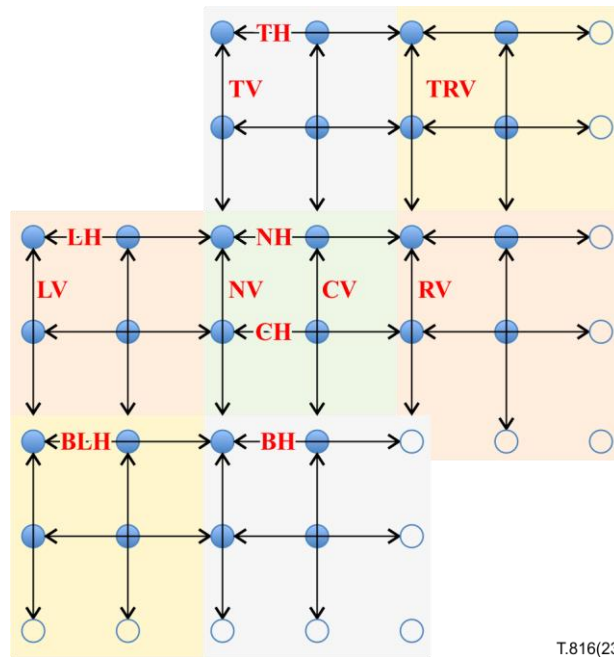
Figure 28 – Neighbouring cells and arcs involved in forming coding contexts for QuadBPT significance decoding in CL band code-blocks
