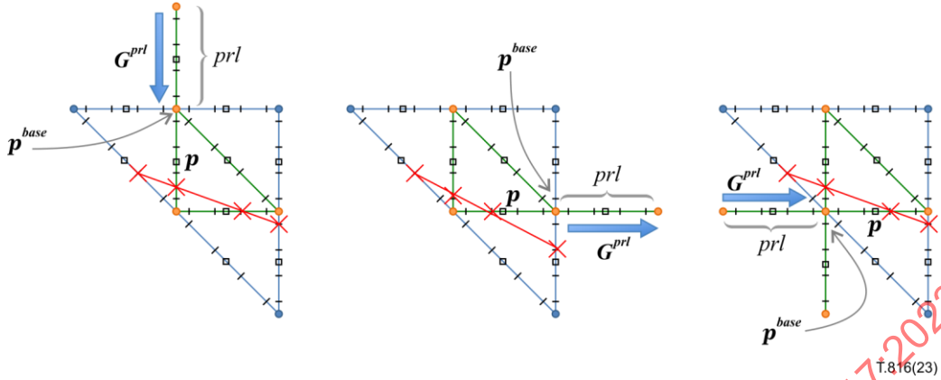
Figure 14 – Examples of arcs p^{rl} parallel in orientation to root arcs centred at p and containing a spatially induced break. Gradient calculated across arc p^{rl} is denoted as G^{prl}
