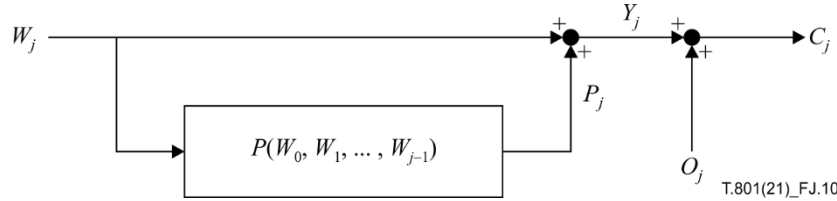
Figure J.10 – Forward irreversible dependency transformation
