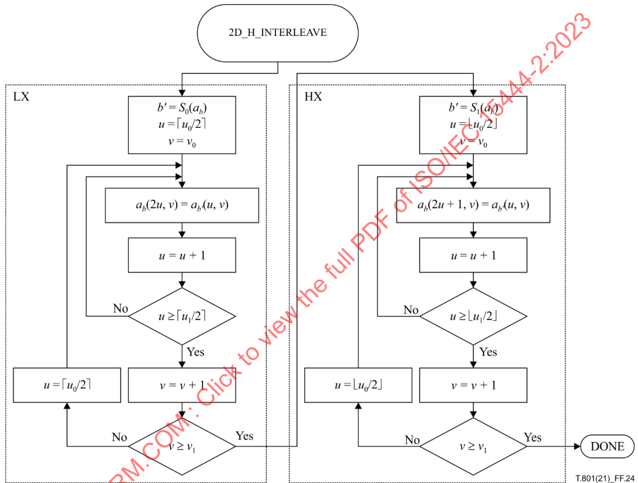
Figure F.24 – The 2D_H_INTERLEAVE procedure
