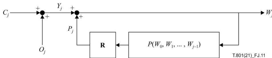
Figure J.11 – Reversible dependency transformation
