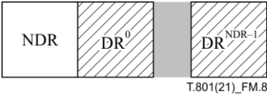
Figure M.8 – Organization of the contents of a Data Reference box
