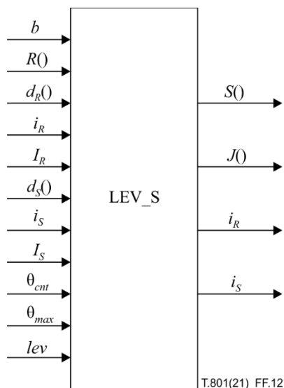
Figure F.12 – Parameters for the LEV_S procedure
