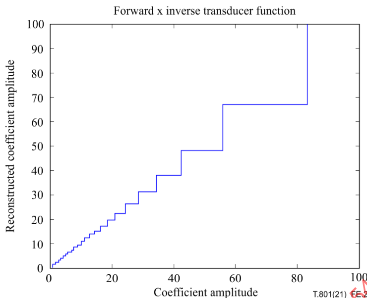
Figure E.2 – Non-uniform quantization for self-contrast masking
