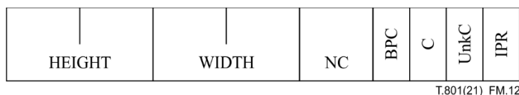
Figure M.12 – Organization of the contents of an Image Header box
