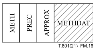
Figure M.16 – Organization of the contents of a Colour Specification box
