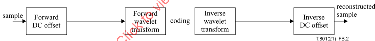
Figure B.2 – Placement of the DC offset without multiple component transformation
