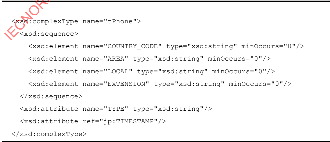
Figure N.55 – Schema of the Phone number type
