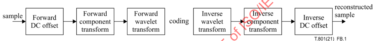
Figure B.1 – Placement of the DC offset with multiple component transformation
