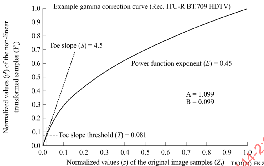
Figure K.2 – Example gamma-type forward non-linear transformation
