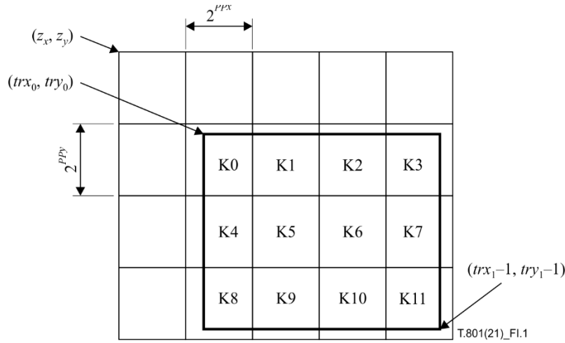
Figure I.1 – Precincts of one reduced resolution (modified Figure B.8 of Rec. ITU-T T.800 | ISO/IEC 15444-1)
