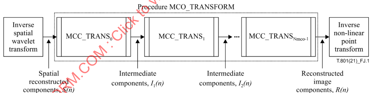
Figure J.1 – Inverse multiple component transformation processing
