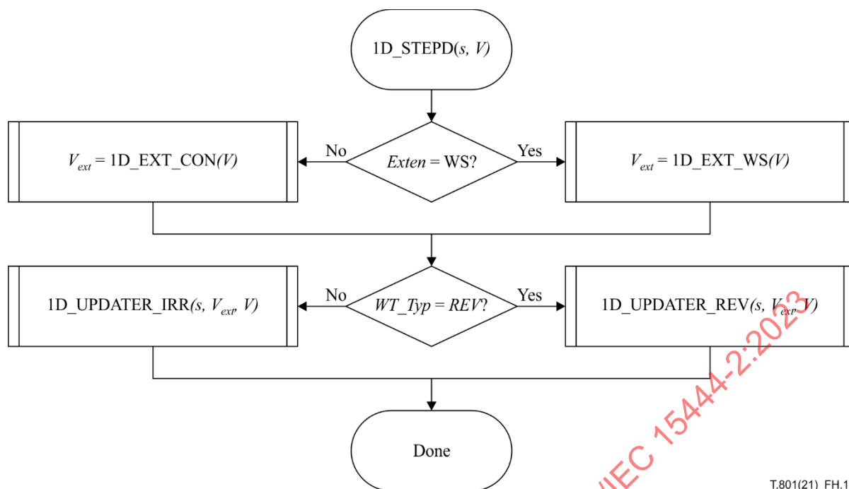
Figure H.13 – Procedure 1D_STEPD
