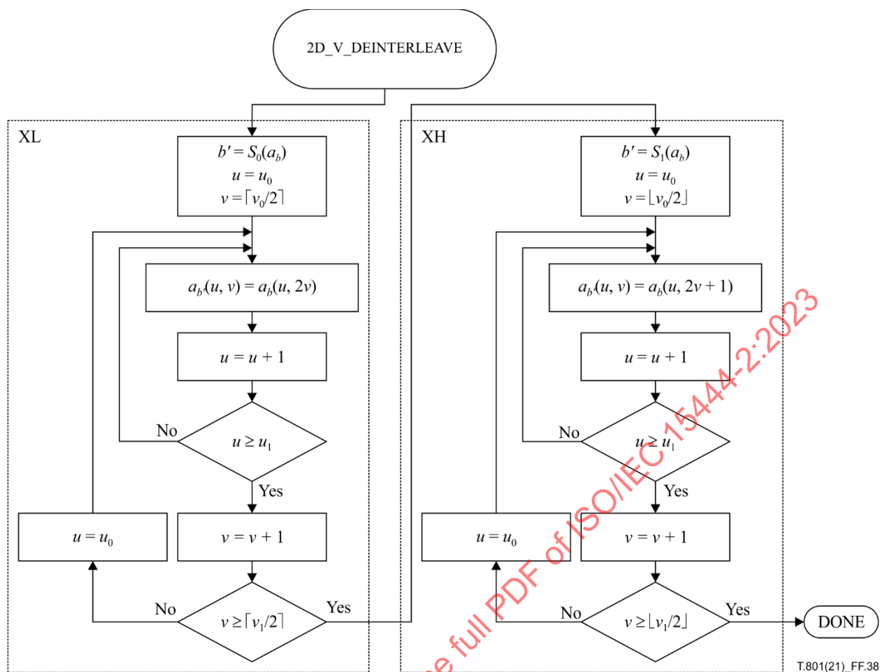
Figure F.38 – The 2D_V_DEINTERLEAVE procedure
