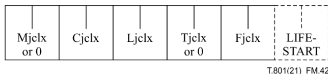
Figure M.42 – Organization of the Compositing Layer Extensions Info box
