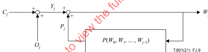
Figure J.9 – Irreversible dependency transformation
