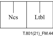
Figure M.44 – Organization of the contents of a Multiple Codestream Offsets box
