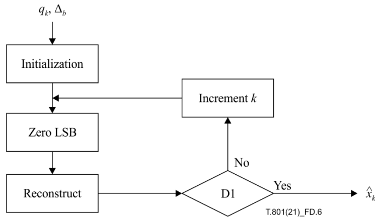
Figure D.6 – Approximate dequantization of TCQ indices
