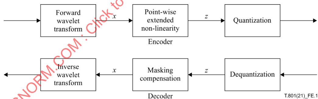
Figure E.1 – System diagram for point-wise extended masking extension
