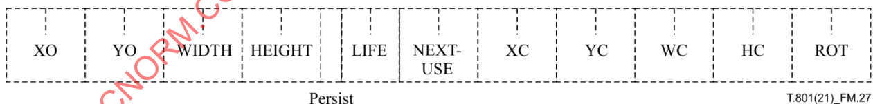
Figure M.27 – Organization of the contents of an INST field within an Instruction Set box
