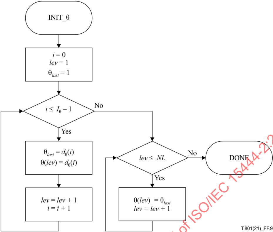
Figure F.9 – Procedure for setting maximum number of sub-levels, \\theta(lev)
