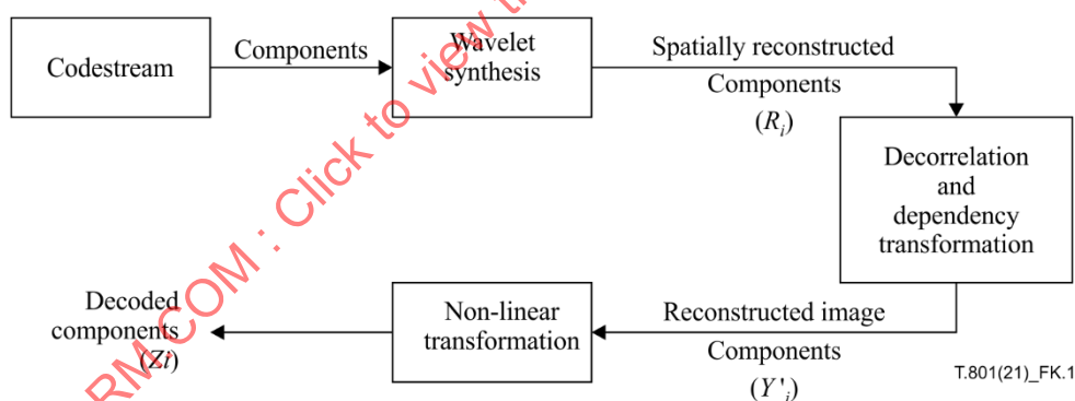
Figure K.1 – Non-linear transformation application during decoding
