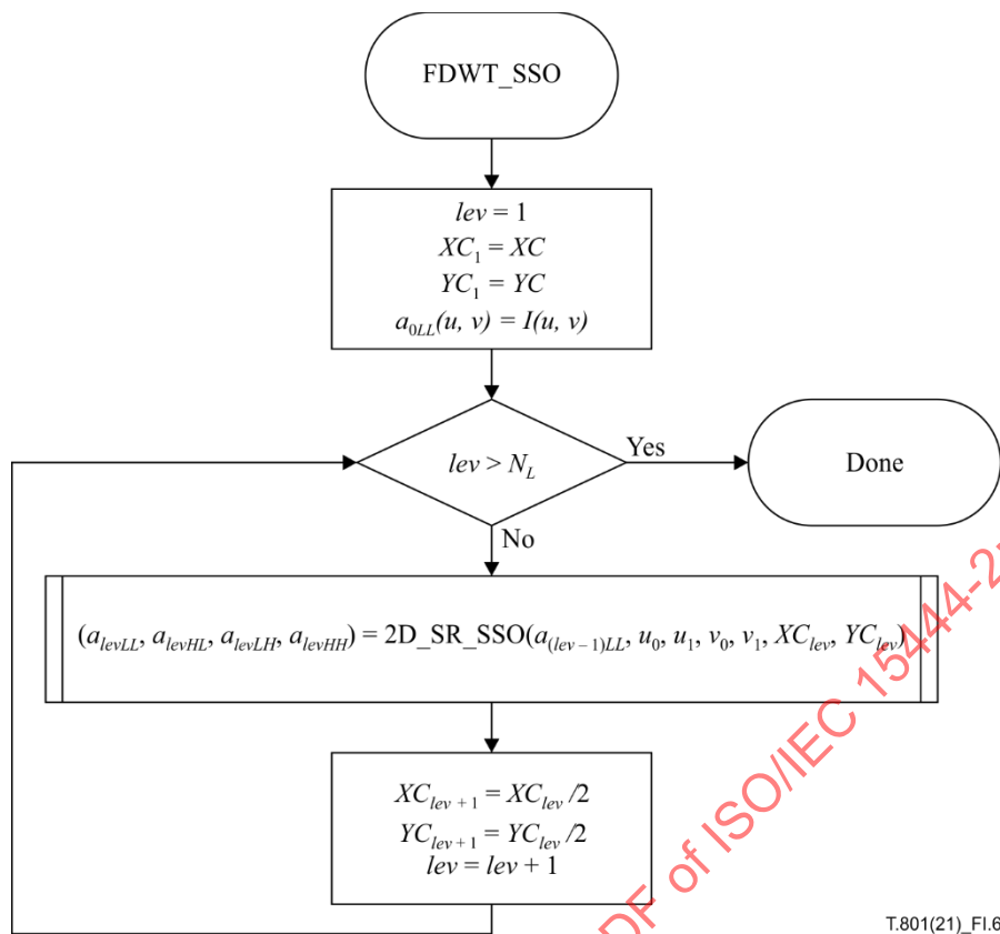
Figure I.6 – The FDWT_SSO procedure
