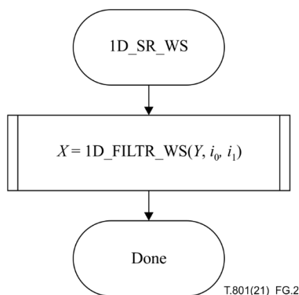
Figure G.2 – The 1D_SR_WS procedure
