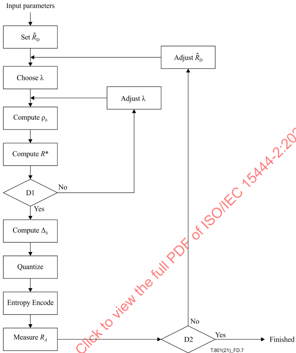
Figure D.7 – Lagrangian rate allocation
