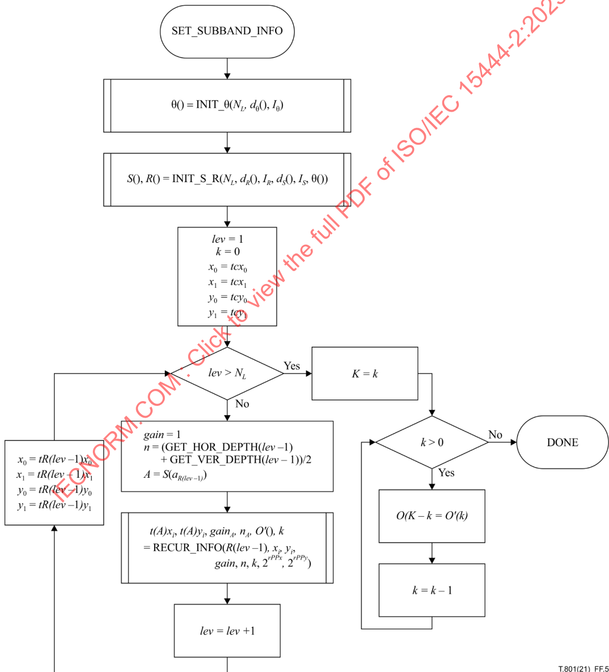
Figure F.5 – The SET_SUBBAND_INFO procedure
