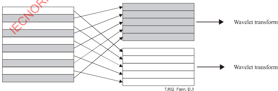
Figure D.3 – Picture structure in field-based coding (topmost line second)
