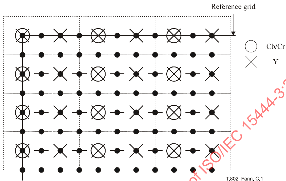
Figure C.1 – 4:2:2 format (co-sited)
