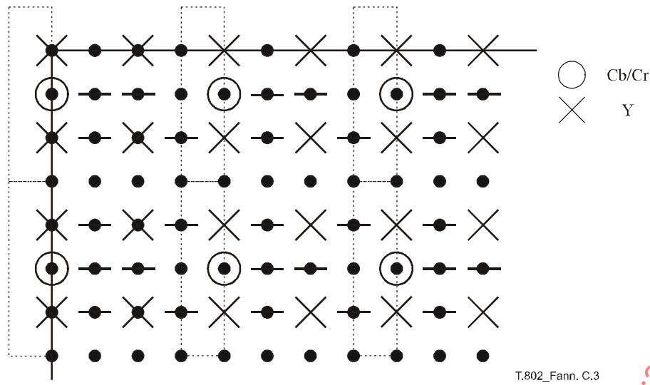
Figure C.3 – 4:2:0 format (co-sited)
