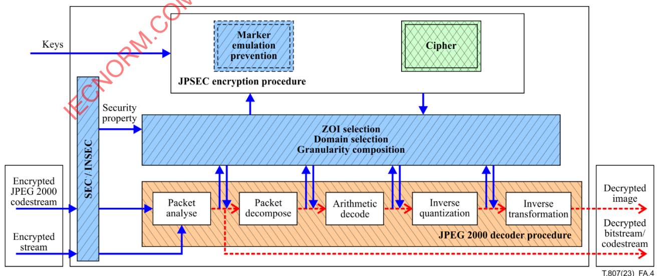
Figure A.4 – Decryption procedure
