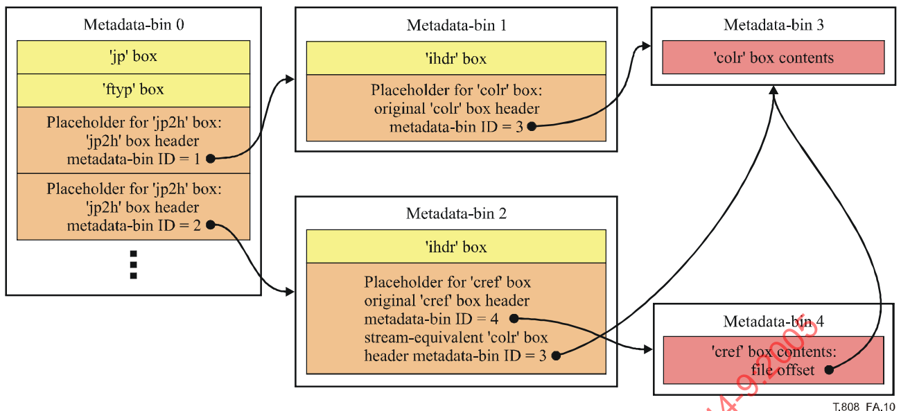
Figure A.10 – Example of the use of stream equivalents
