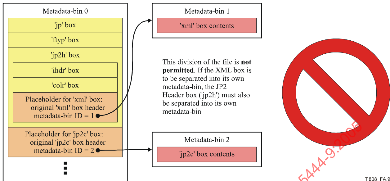
Figure A.9 – An illegal division of the file into metadata-bins
