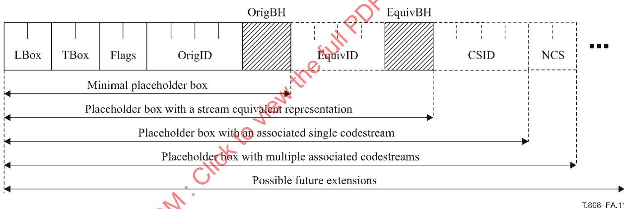
Figure A.11 – Placeholder box structure
