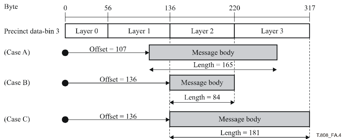
Figure A.4 – Example precinct data-bin
