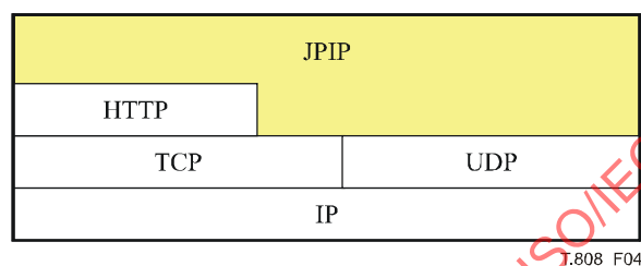
Figure 4 – JPIP protocol stack
