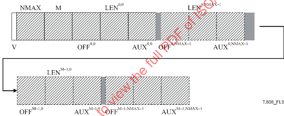
Figure I.5 – Organization of the contents of a Fragment Array Index box
