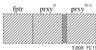
Figure I.11 – Organization of the contents of a File Index box
