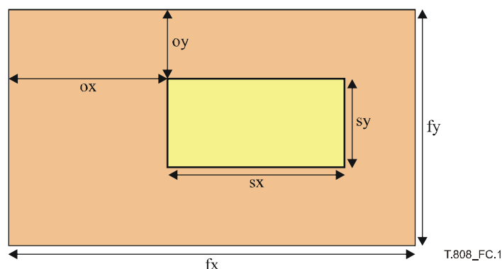
Figure C.1 – Desired region within an image
