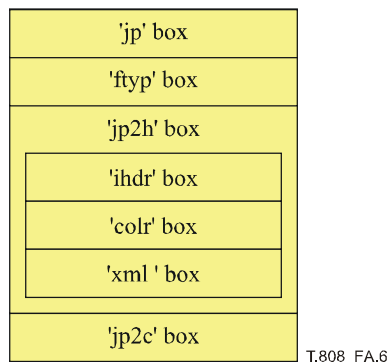
Figure A.6 – A sample JP2 file
