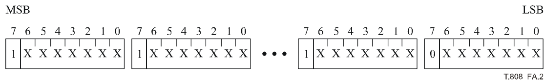
Figure A.2 – VBAS structure
