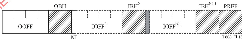
Figure I.13 – Organization of the contents of a Proxy box
