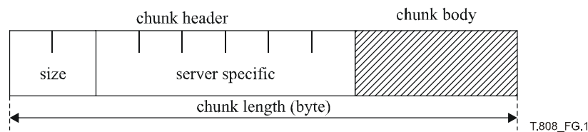
Figure G.1 – Response data structure on http-tcp connection
