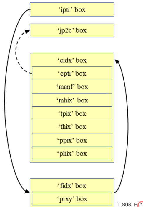
Figure I.1 illustrates an example JPEG 2000 file containing JPIP index boxes:
