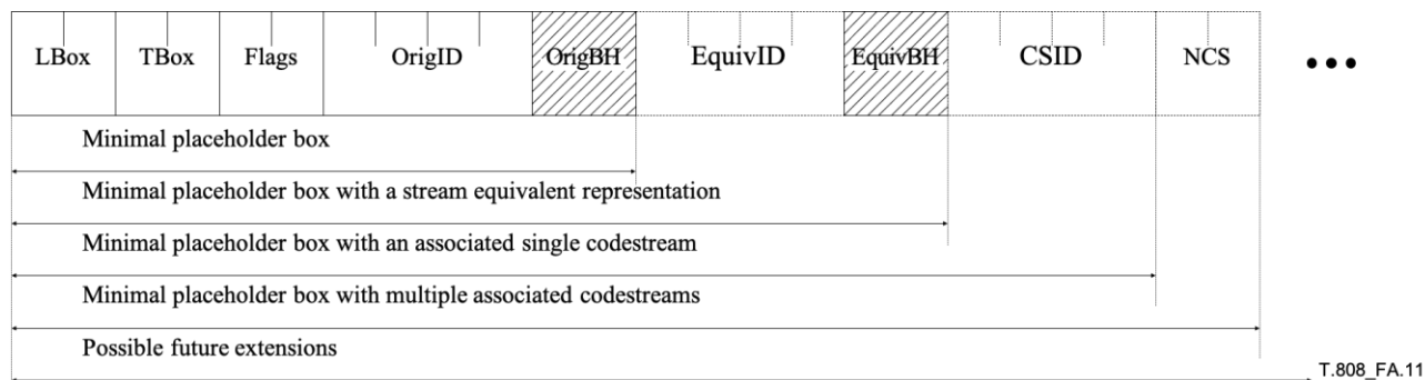
Figure A.11 – Placeholder box structure
