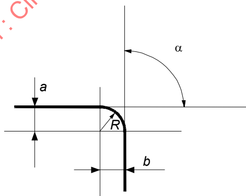
Figure 4 — Rounded corner
