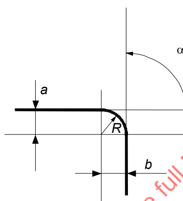
Figure 4 — Rounded corner
