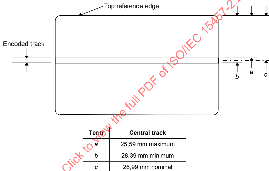
Figure 5 — Position for TFC.1 central track
