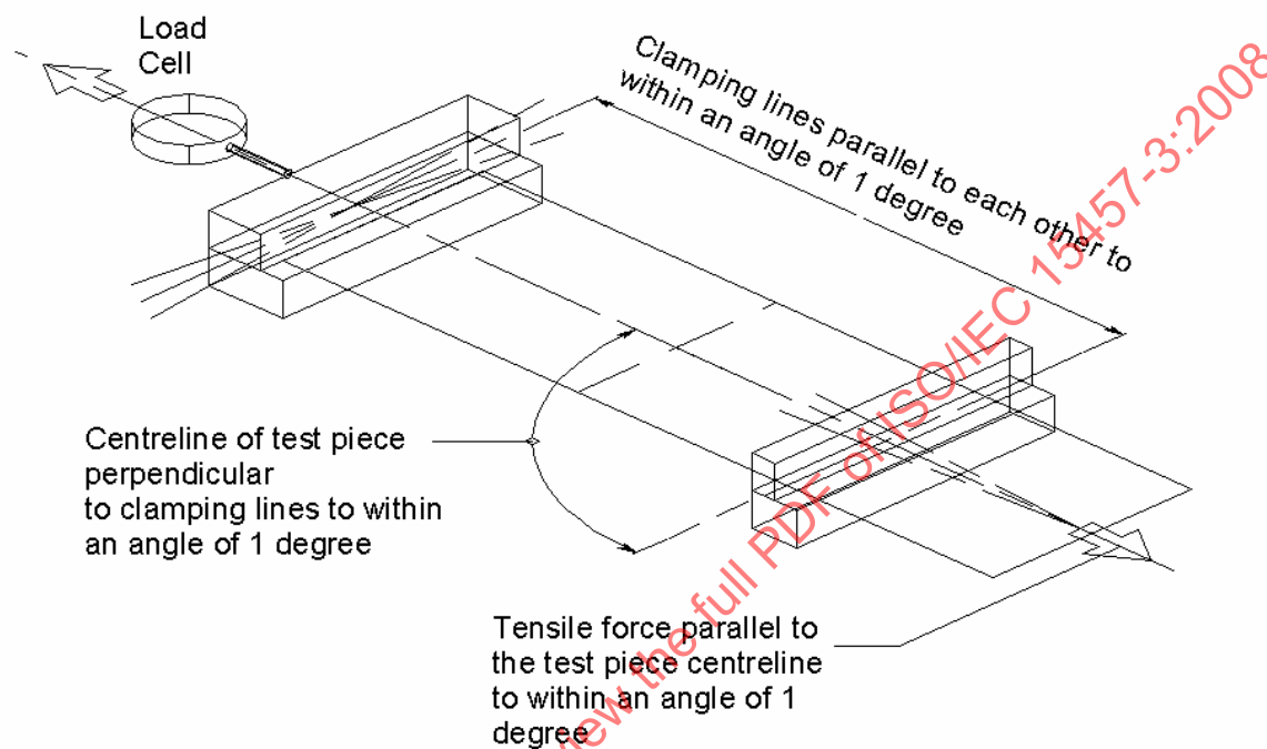
Figure 1 — Test arrangement for separation force
