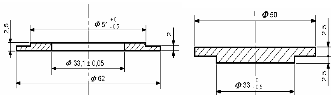
A: annular disc receiving the material — brass
