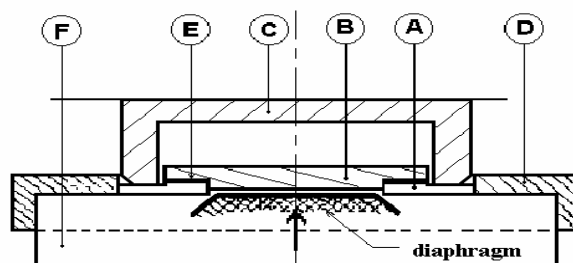
D: ring for centring on the burst tester — mild steel
