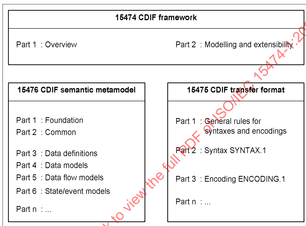
Figure 5 – Architecture of the CDIF family of standards
