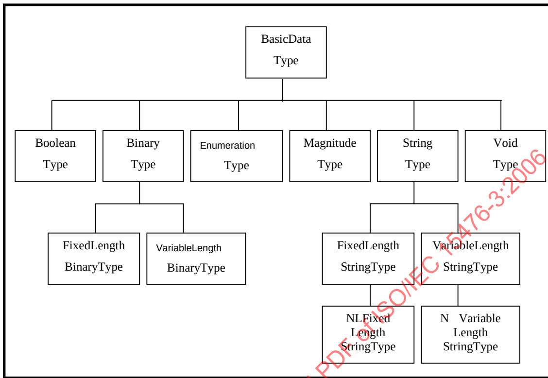
Figure 10 – BasicDataType Subtypes
