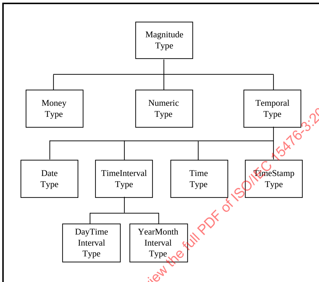
Figure 11 – MagnitudeType Subtypes
