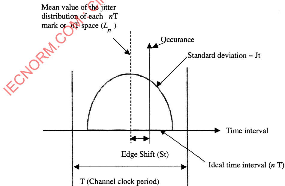
Figure J.1 - Measured timing distribution yielding Jitter J(t) and Edge Shift S(t)
