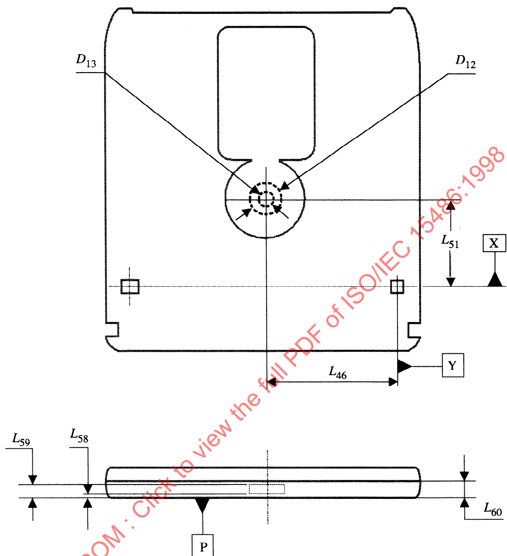
Figure 13 - Capture cylinder
