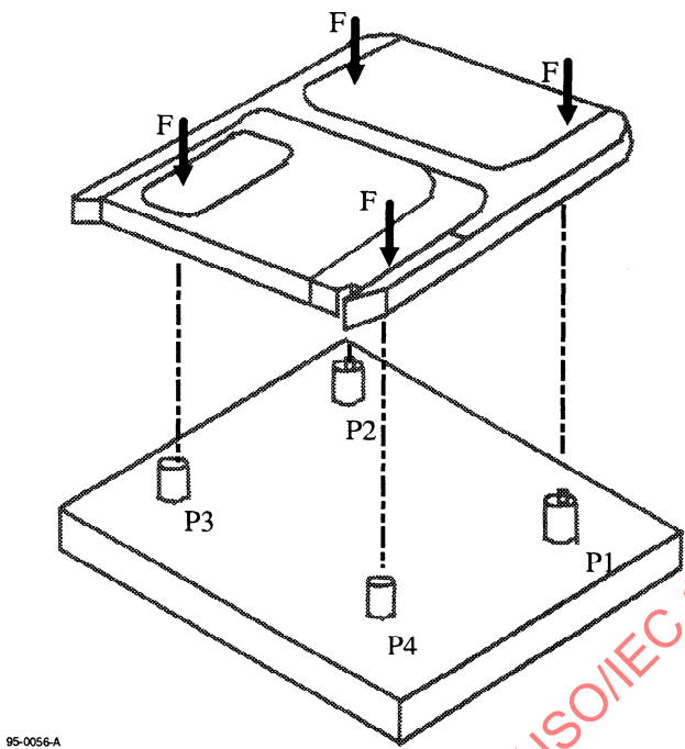
Figure C.1 - Compliance gauge
