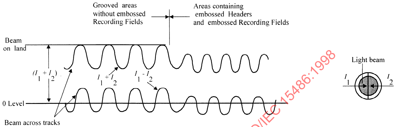
Figure 23a - Signals from grooves in the tracking Channel
