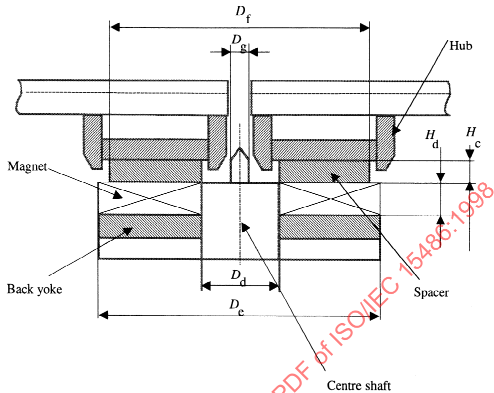
Figure D.1 - Test device for the clamping characteristic of the hub
