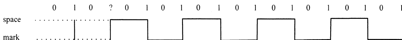
Figure 18 - Postamble pattern
