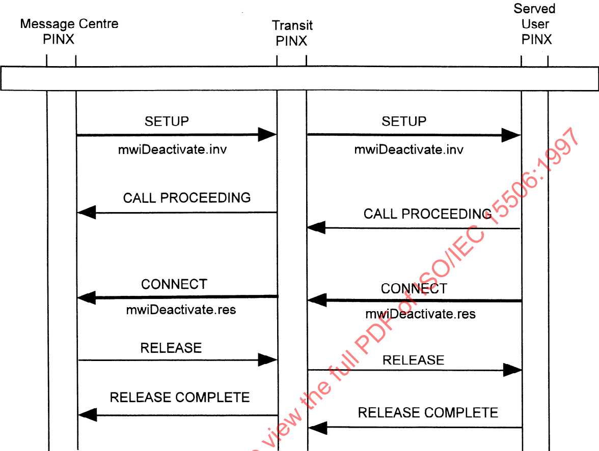
Figure B.2 - Example of deactivation of SS-MWI
