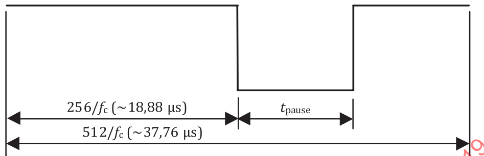
Figure 9 — End of frame for either mode
