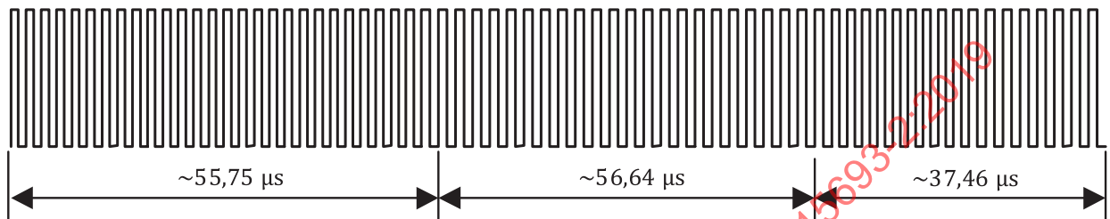
Figure 15 — Start of frame when using two subcarriers
