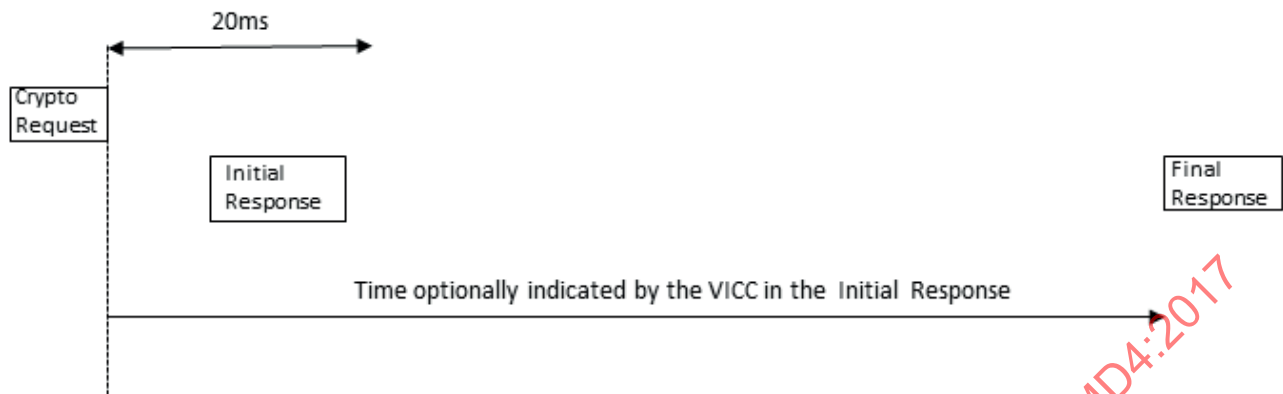
Figure — Amd 4.3 — VICC in-reply process - Asynchronous mode
