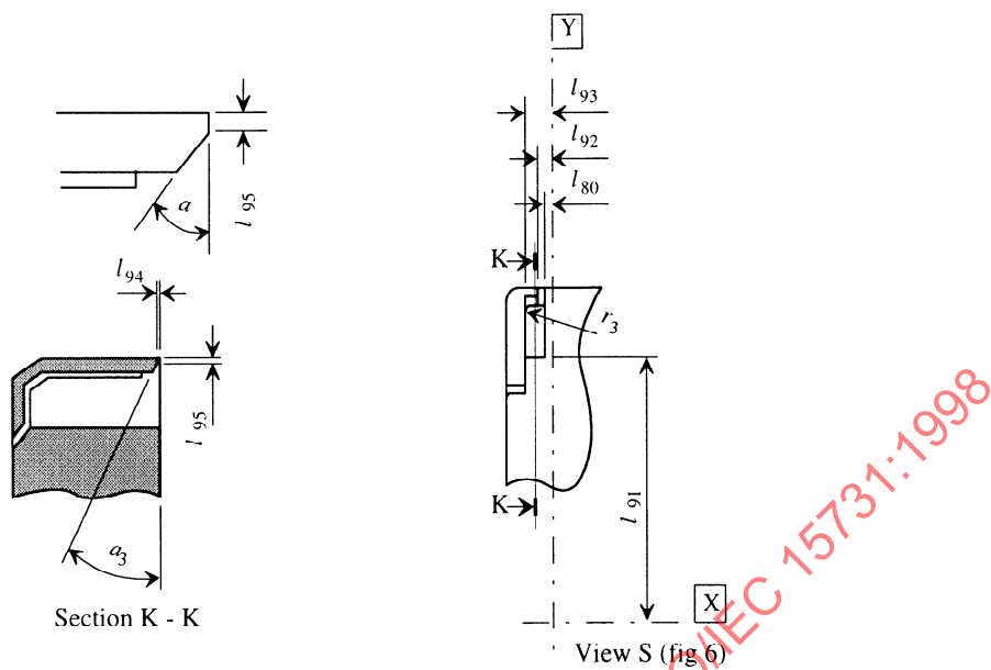
Figure 11 - Lid opening insertion channel of Type S cassette
