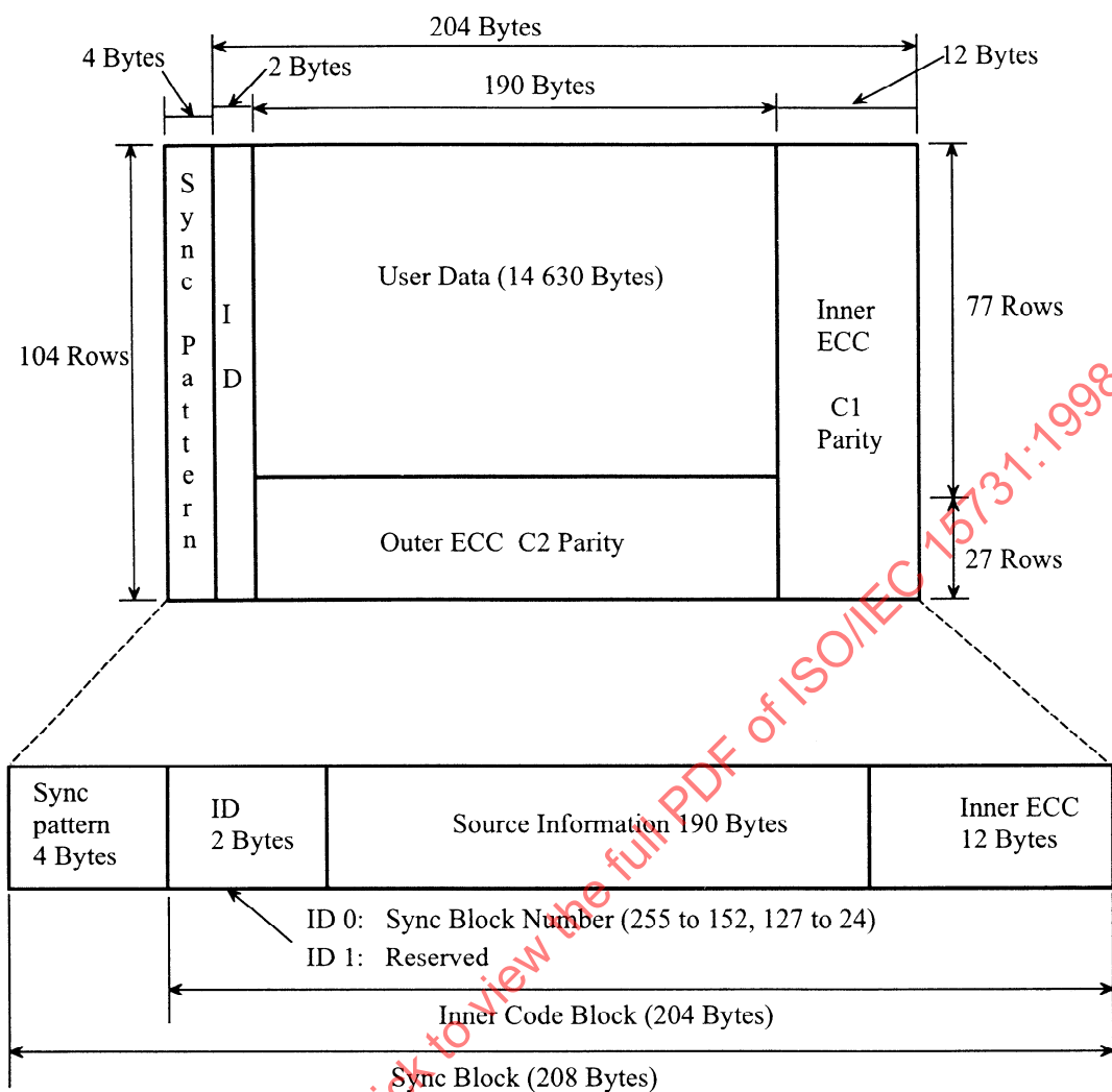
Figure 46 - Sync Block
