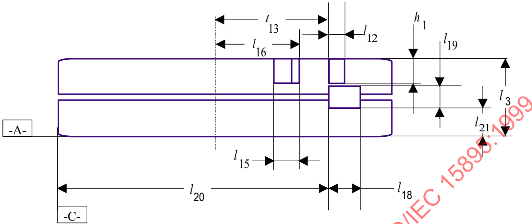
Figure 9 - Right side
