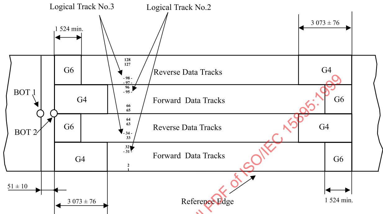
Figure 23 - Layout of the tracks of the Data Area
