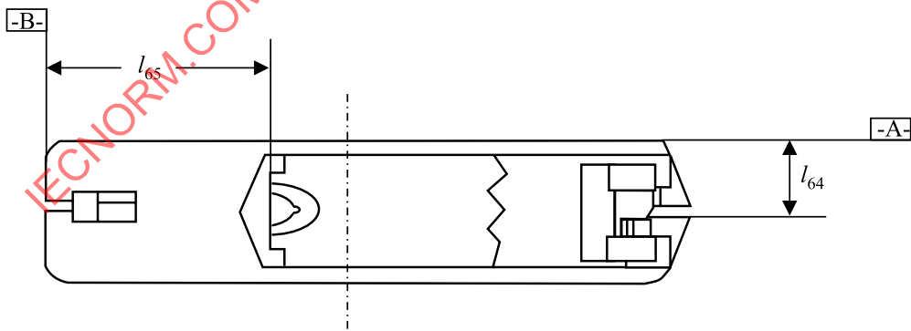
Figure 17 - Front side
