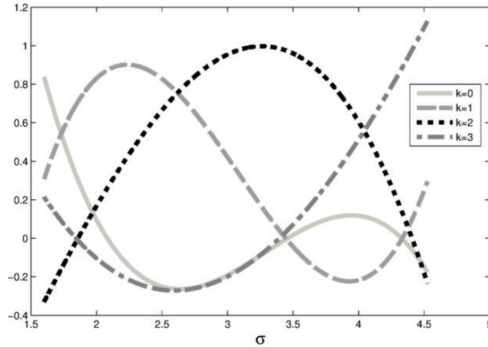
Figure 1 — Polynomial weights for approximating the scale-space function
