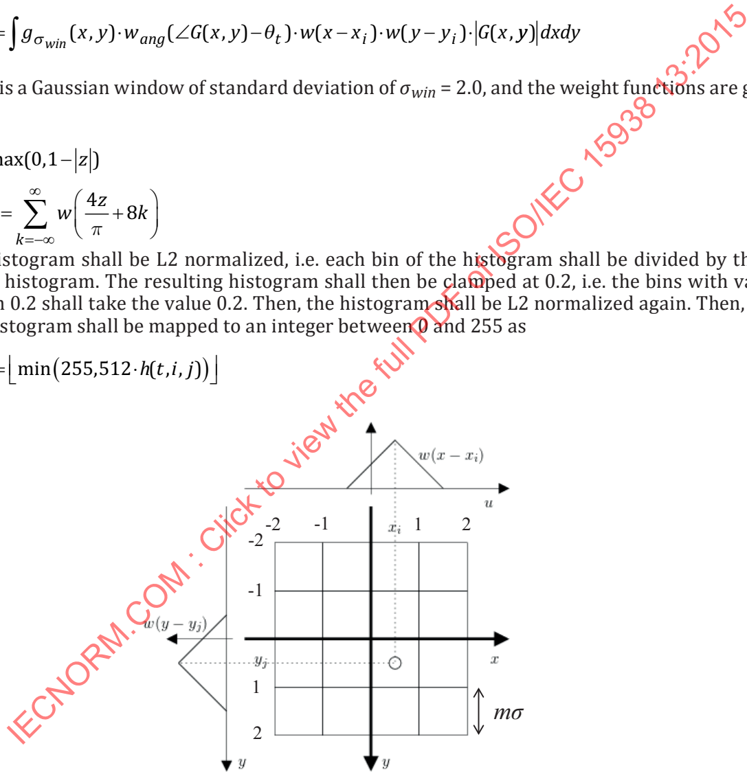
Figure 6 — Local feature descriptor construction
