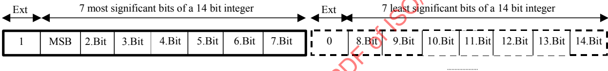
Figure 1 — Informative example for the vuimbsbf8 data type
