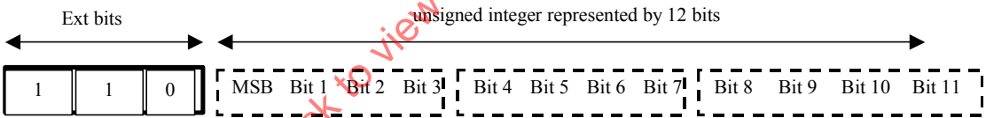
Figure 2 — Informative example for the vuimbsbf5 data type
