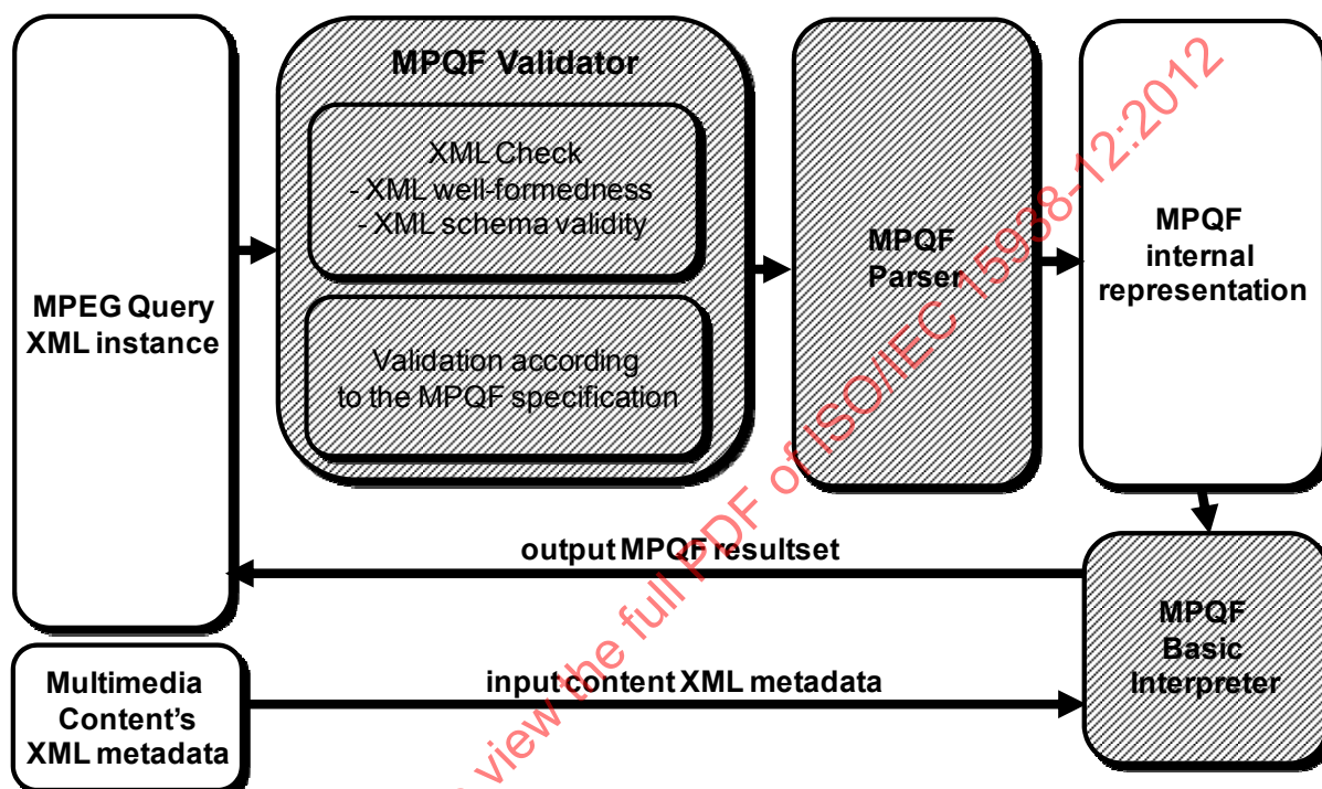
Figure 6 — Reference/utility software architecture
