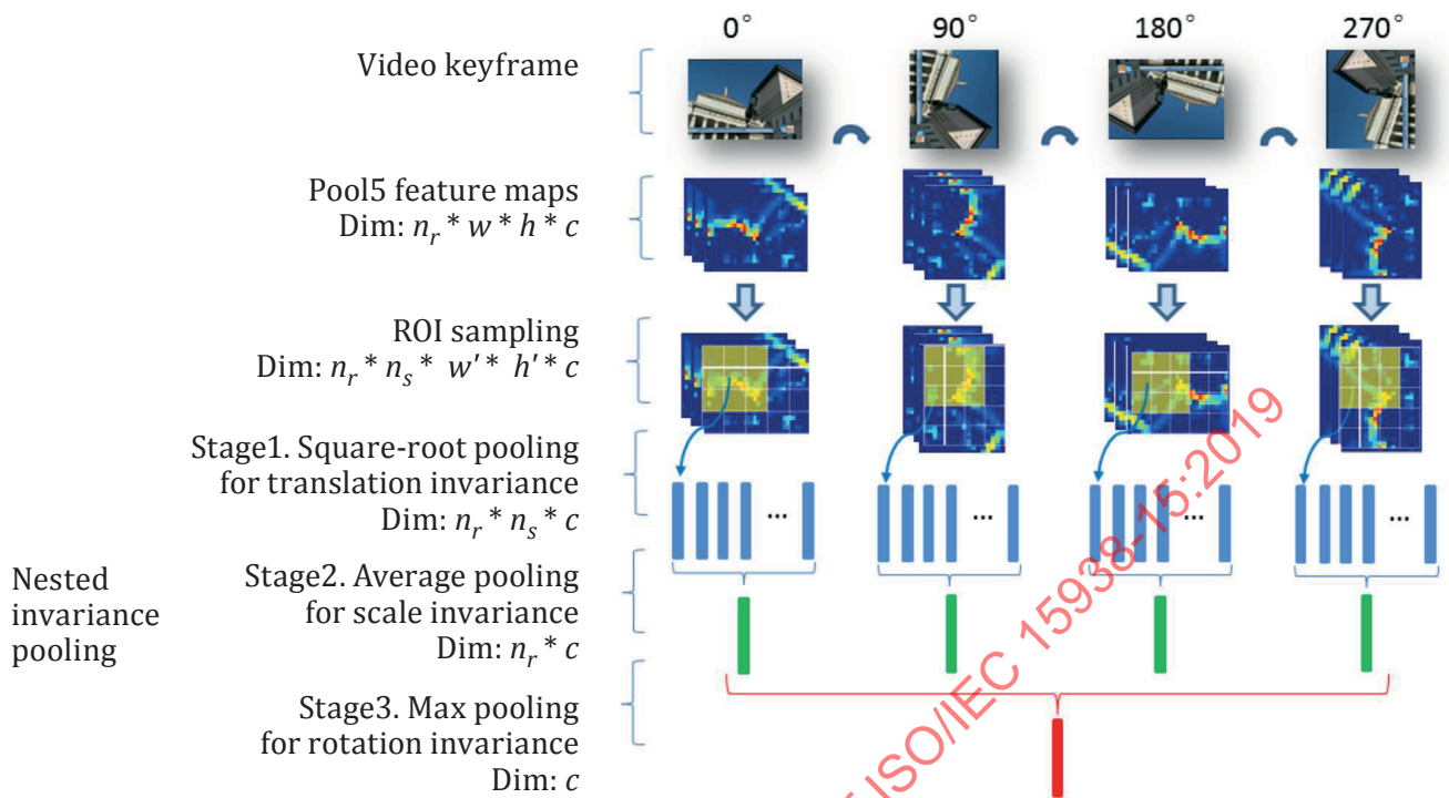
Figure 1 — Nested invariance pooling on feature maps from pool5 layer of VGG-16 network ( n_r = 4 )
