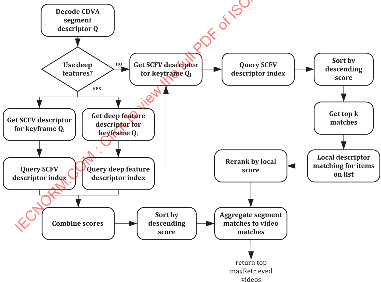
Figure 3 — CDVA retrieval pipeline
