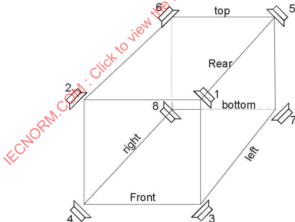
Figure AMD1-2 - Scheme and channel number for a 3D speaker arrangement (example)
