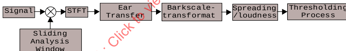
Figure 13 — Loudness based Silence Detector
