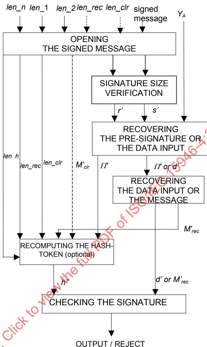
Figure 2 — Signature verification process
