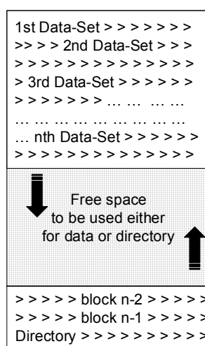
Figure 5 — Logical Memory Schematic - Directory Structure
