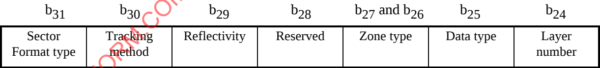
Figure 18 - Sector Information of the Identification Data (ID)
