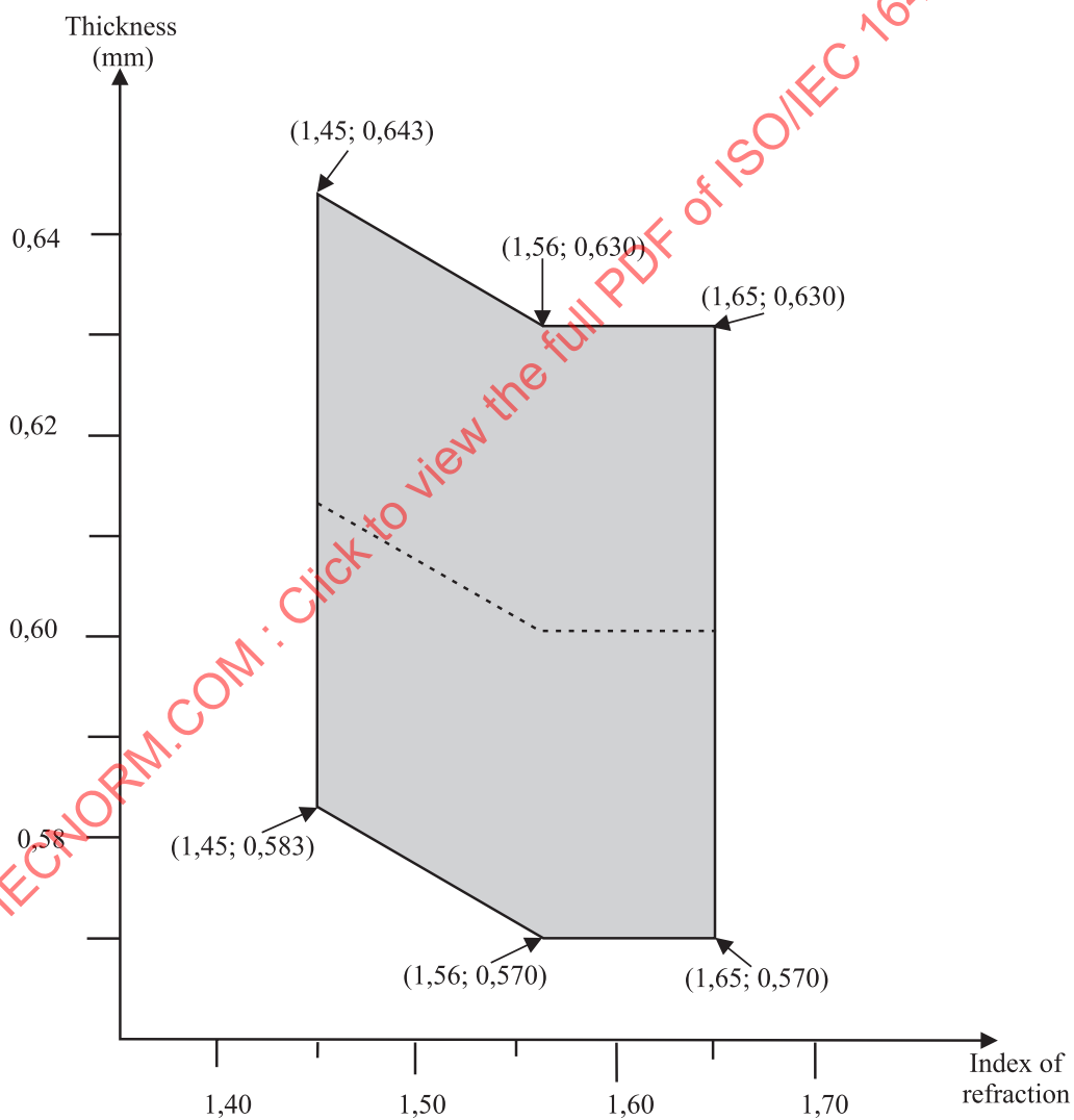
Figure 8 - Rim area
