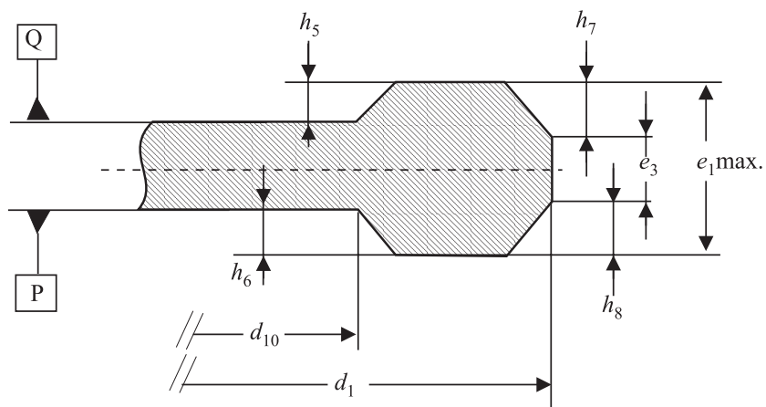
Figure 8 - Rim area
