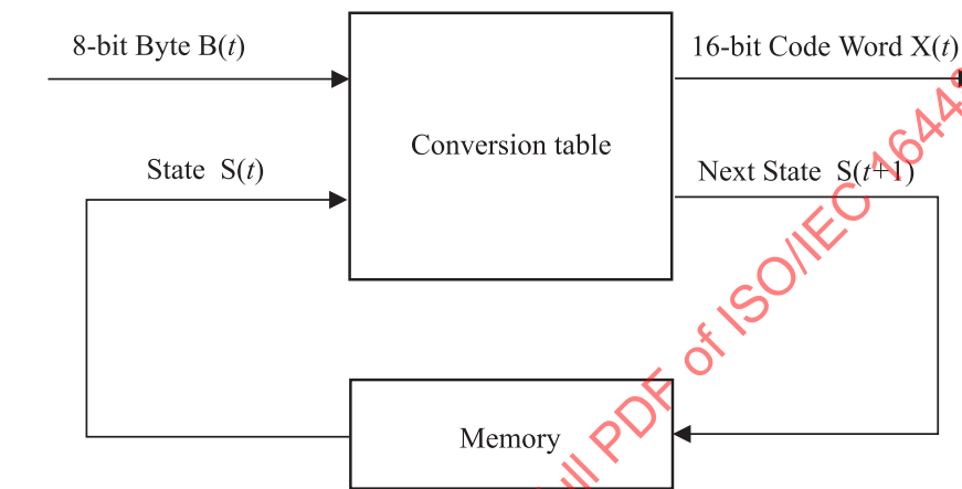
Figure G.1 - Code Words generation
