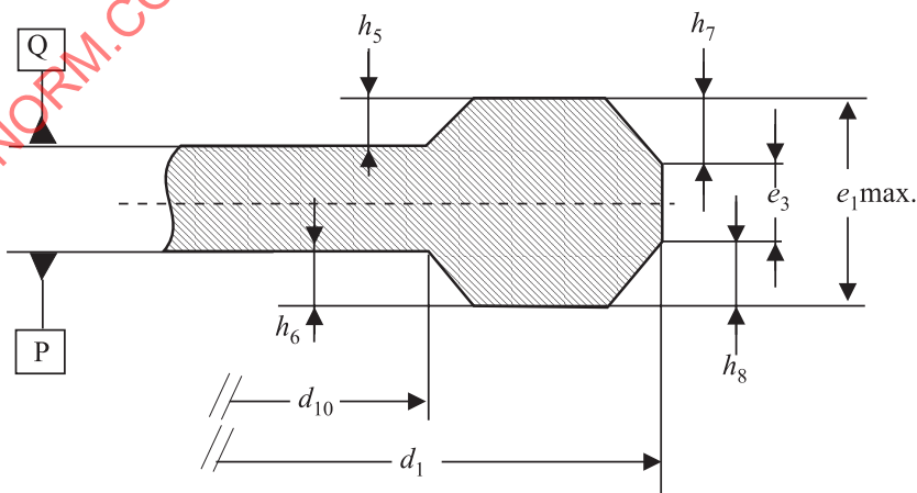
Figure 7 - Areas of the disk
