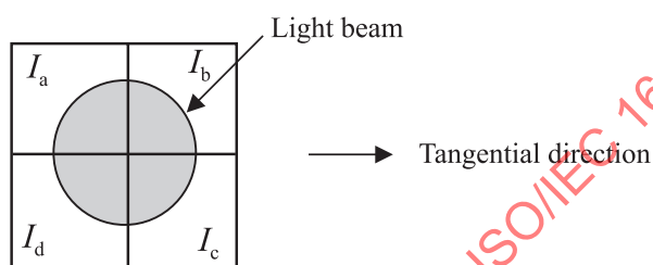
Figure 12 - Cross-track signal
