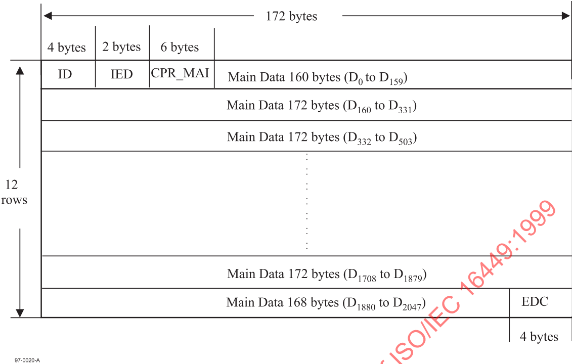
Figure 16 - Data Frame
