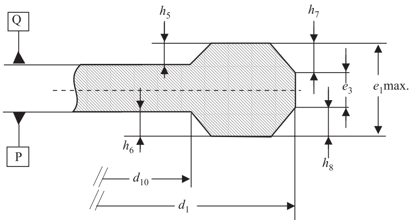
Figure 8 - Rim area
