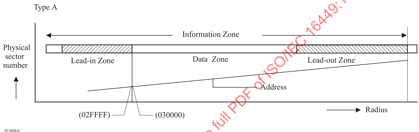
Figure 24 - Physical Sector numbering on Type A
