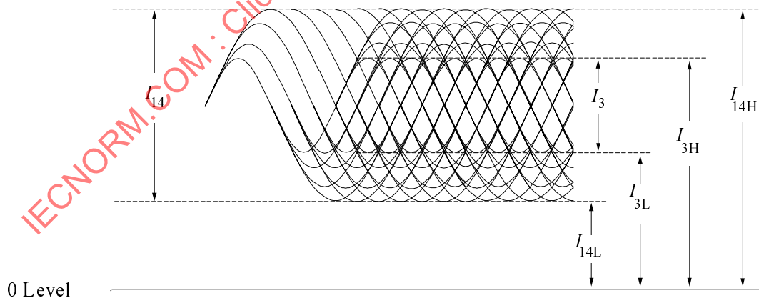
Figure 11 - Modulated amplitude
