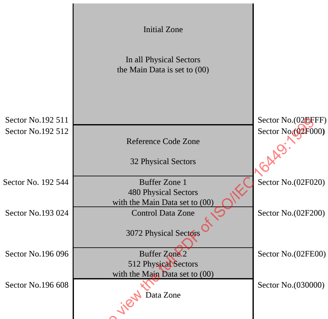
Figure 27 - Lead-in Zone
