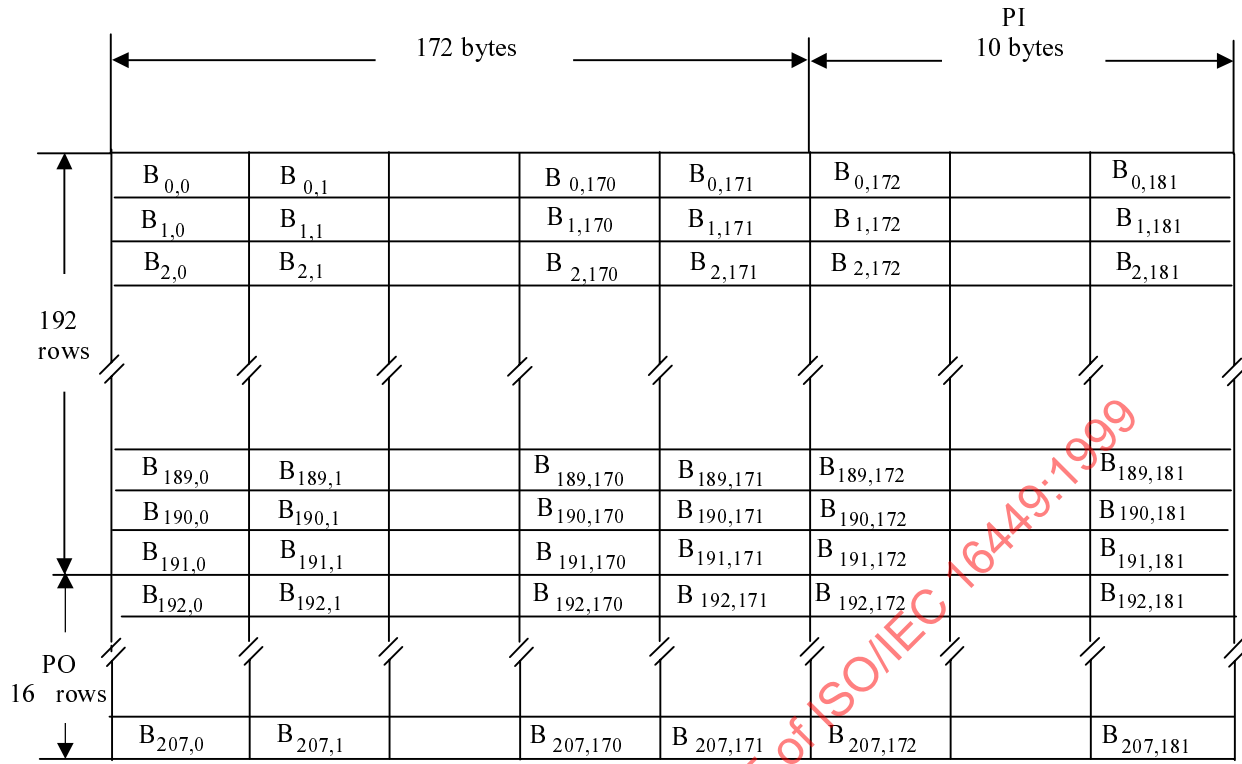
Figure 20 - ECC Block
