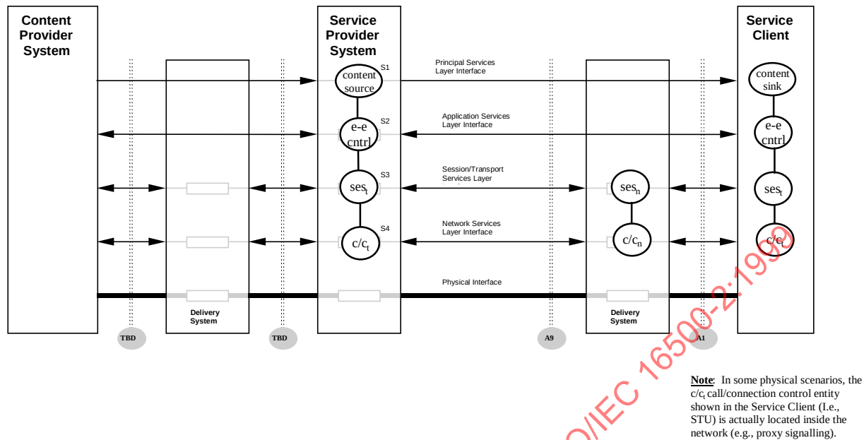
Figure 9.2-2 — Mapping of Dynamic Modeling Functional Entities to Systems Reference Model
