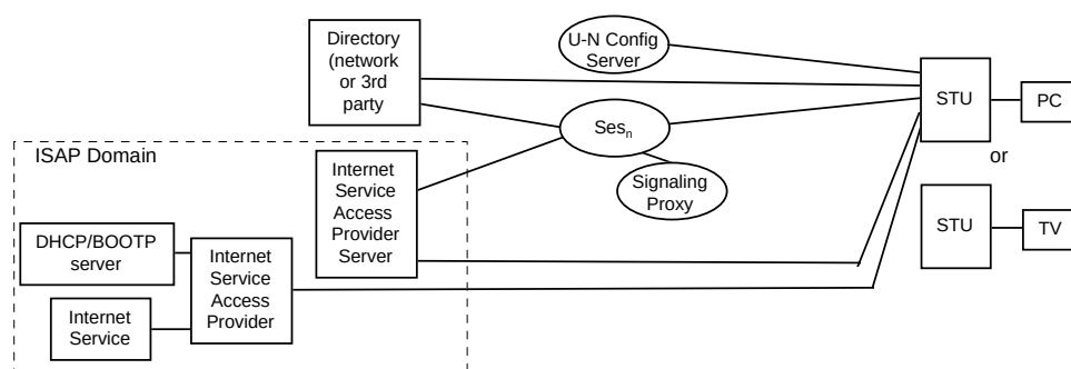
Figure 9.5-22 - System level Connectivity for Integrated Internet Scenario 4
