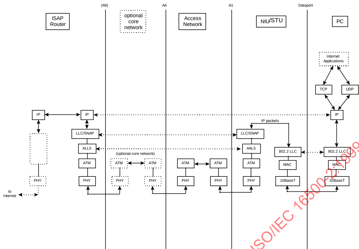
Figure 9.5-26 - Protocol Stacks for Upstream (All Cases) and Downstream (for ATM end-to-end)
