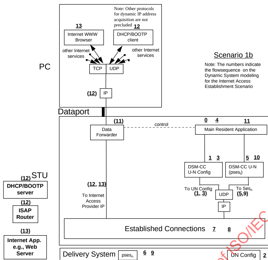
Figure 9.5-12 - STU and PC Level Entities for Direct Internet Access Scenario 1b
