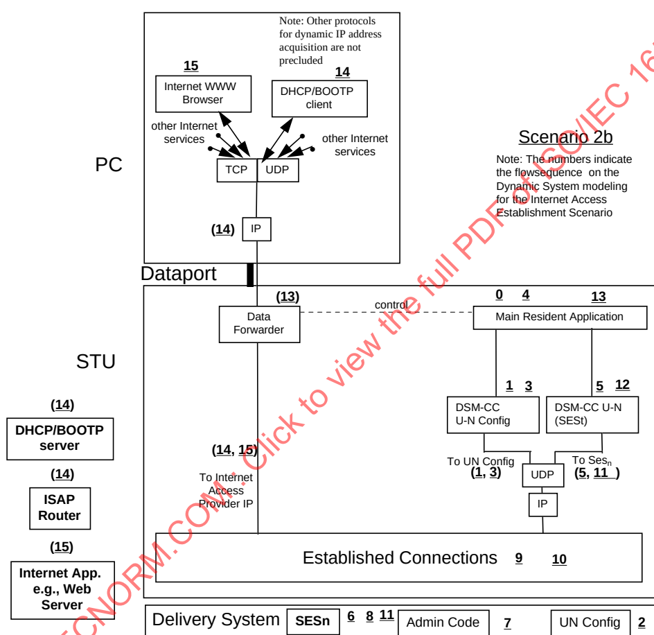
Figure 9.5-18 - STU and PC Level Entities for Direct Internet Access Scenario 2b
