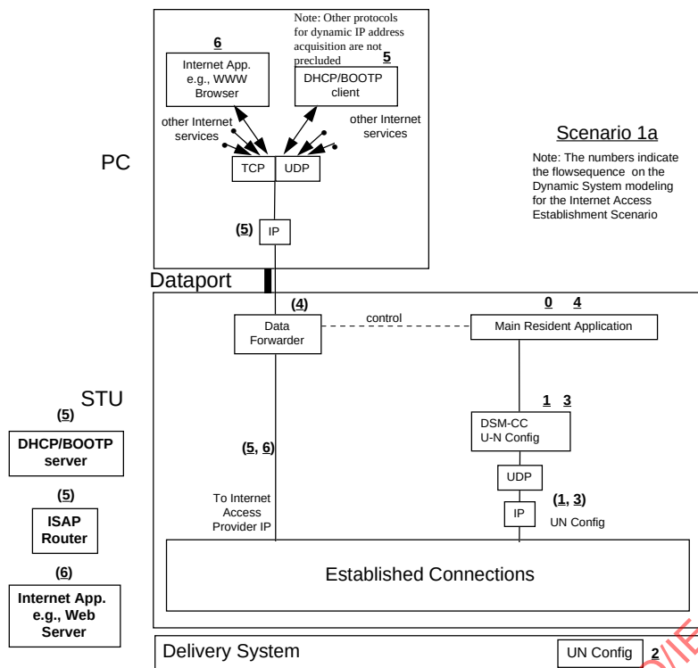
Figure 9.5-8 – STU and PC Level Entities for Direct Internet Access Scenario 1a
