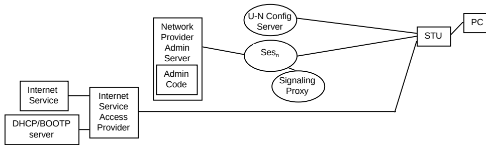
Figure 9.5-14 - System level Connectivity for Direct Internet Scenario 2a
