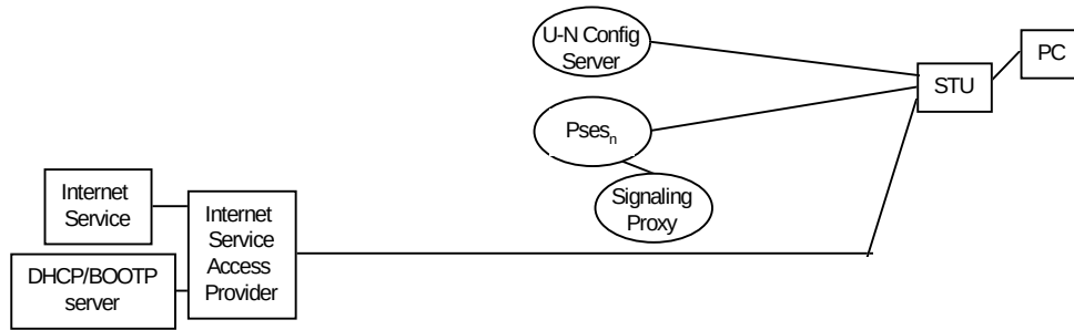
Figure 9.5-10 - System level Connectivity for Direct Internet Scenario 1b
