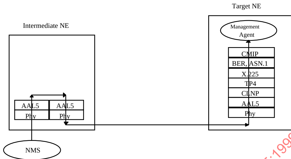
Figure 10.8 — Management Information flow for ATM based NMS
