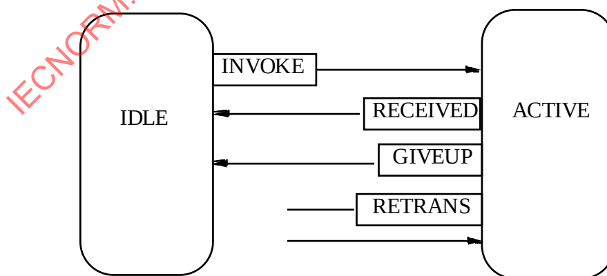
Figure 8.6 — STB state machine model
