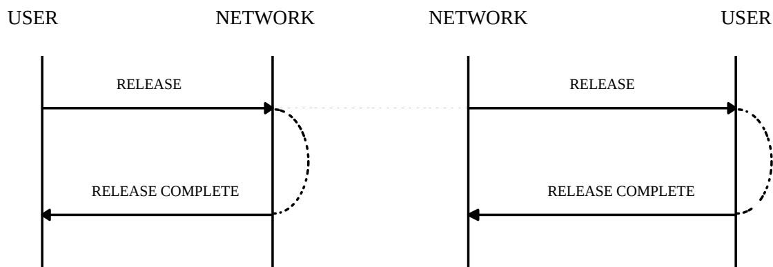
Figure 9.6 — Call clearing message sequence
