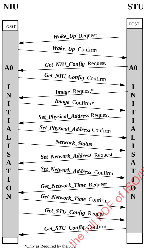
Figure 12.1— A0 Initialization Flow
