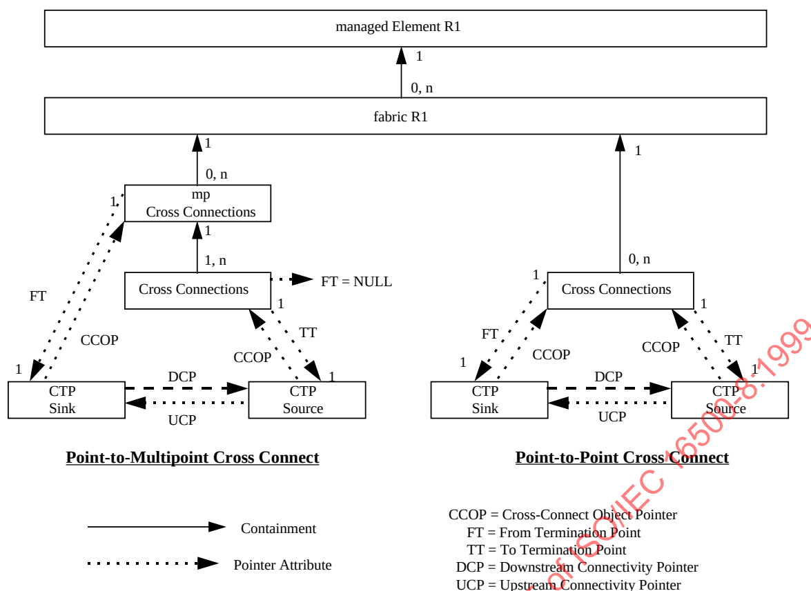
Figure 7-10 — Entity Relationship of Cross-Connect
