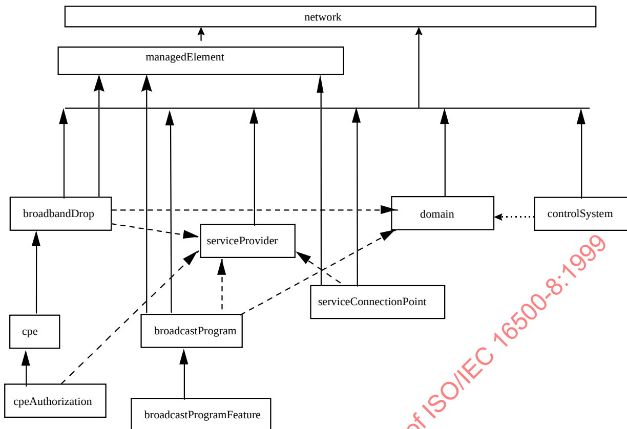
Figure 8-11 — Naming and Relationship Diagram for Information Model
