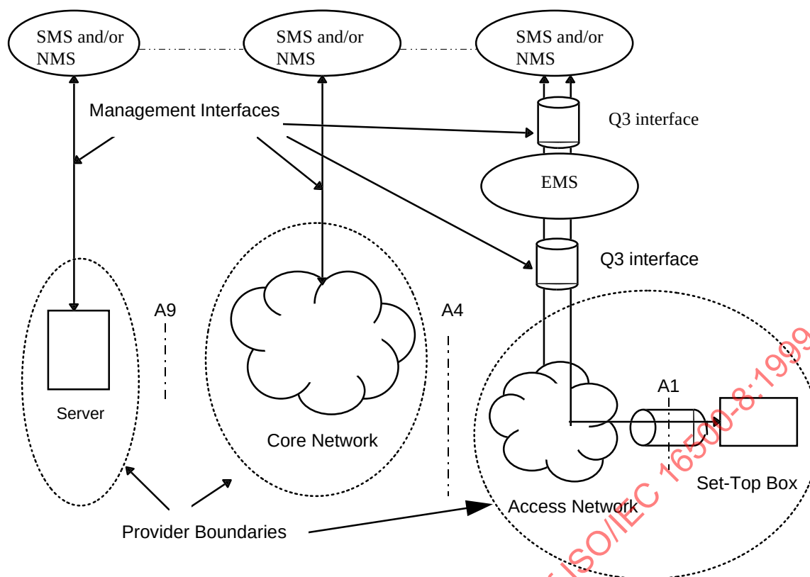
Figure 7-3 — Network Management Architecture - An Example
