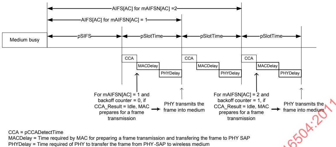
Figure 16 — PCA timing relationships
