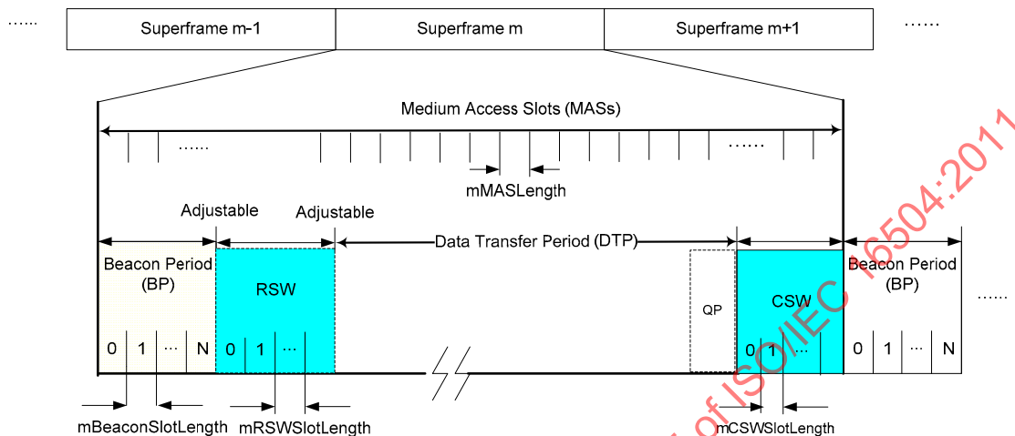
Figure 5 — MAC superframe structure
