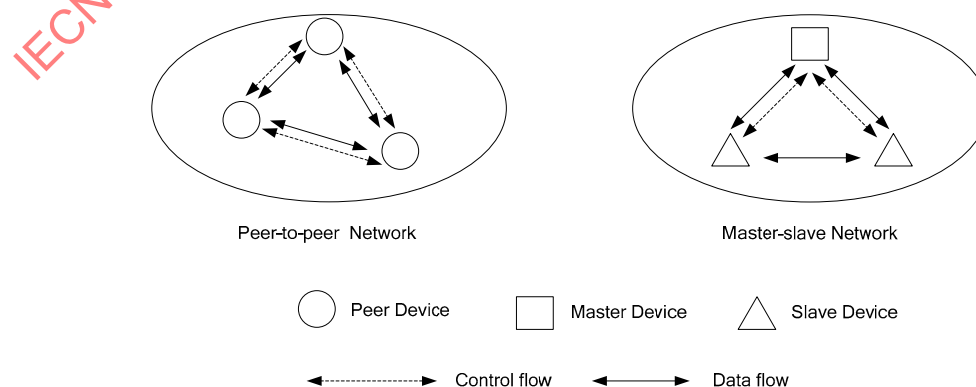
Figure 1 — Basic Network Formation
