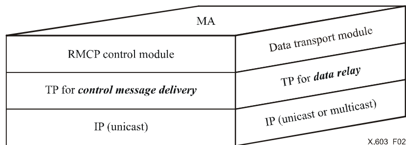
Figure 2 – Inside of Multicast Agent (MA)
