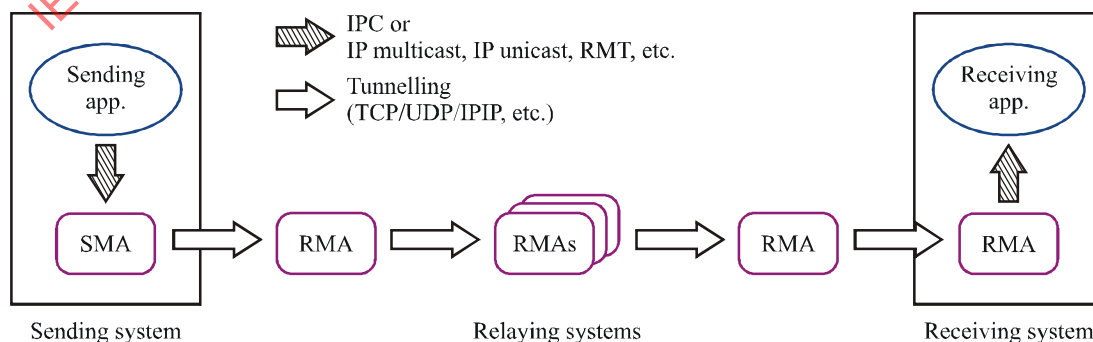
Figure 4 – RMCP data transport model
