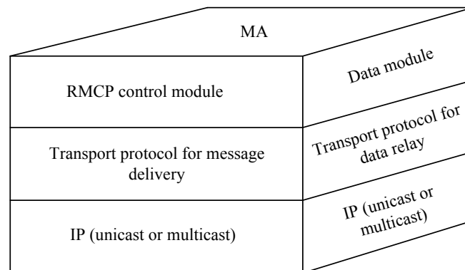
Figure 3 – Protocol stack of the MA
