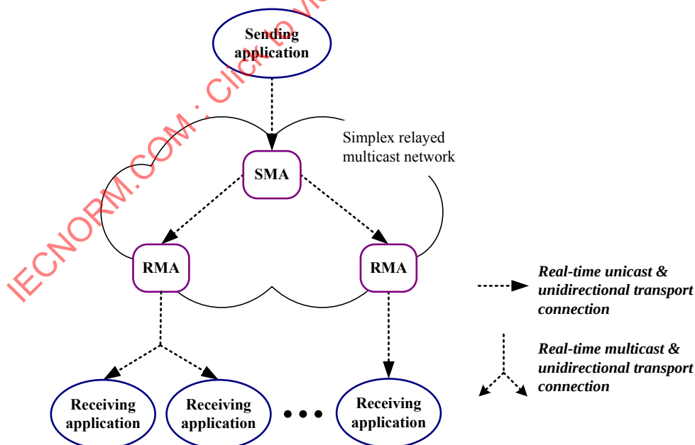
Figure 6 – Simplex real-time data delivery model
