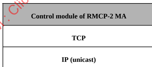
Figure 3 – Protocol stack of MA's control module
