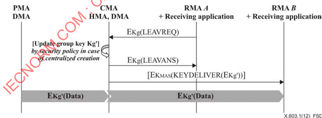
Figure 50 – Secure leave of RMA
