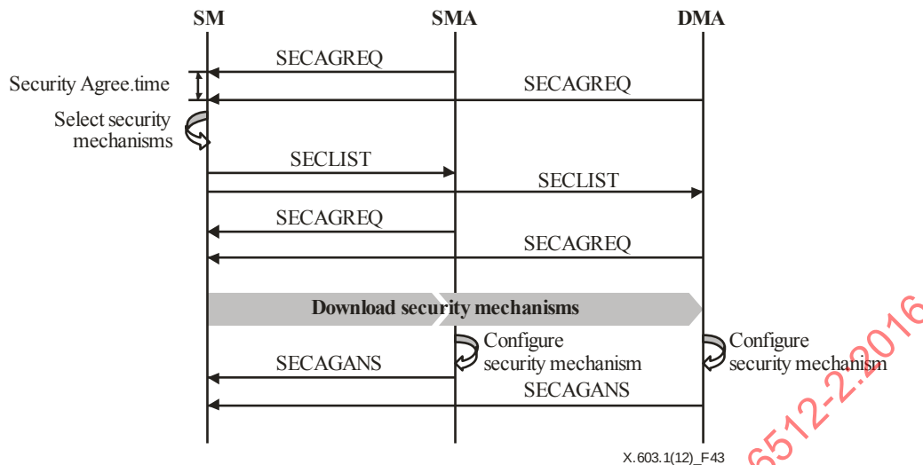
Figure 43 – Security agreement of DMA and SMA
