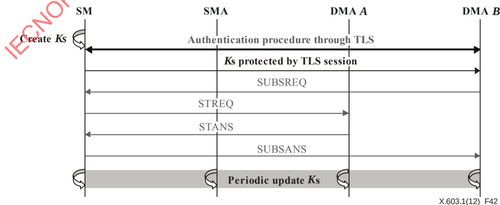
Figure 42 – Session key management
