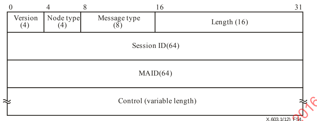
Figure 54 – Common RMCP-2 message format
