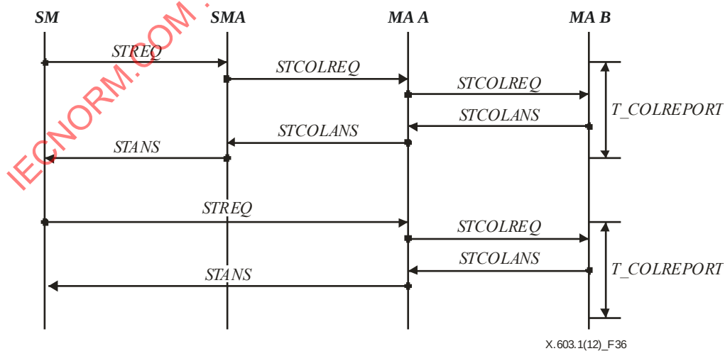
Figure 36 – Tree monitoring by collecting a status report
