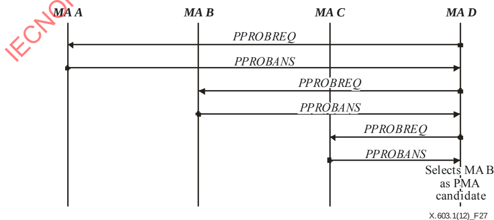
Figure 27 – Neighbour discovery in a unicast network
