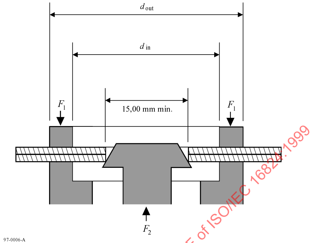
Figure A.2 - Clamping and chucking conditions
