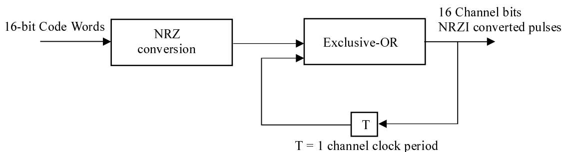
Figure 15 - NRZI conversion
