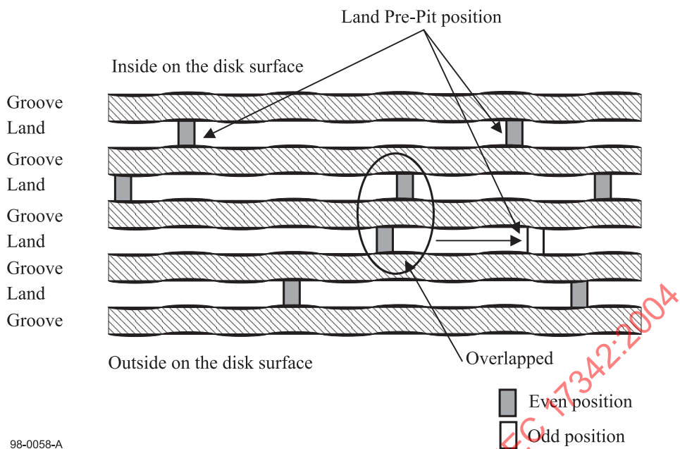
Figure 46 - Layout of land Pre-pit positioning
