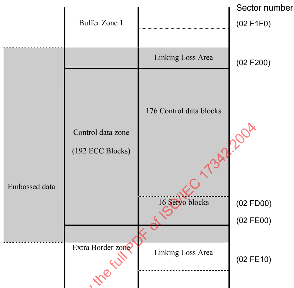
Figure 39 - Structure of Control Data Zone
