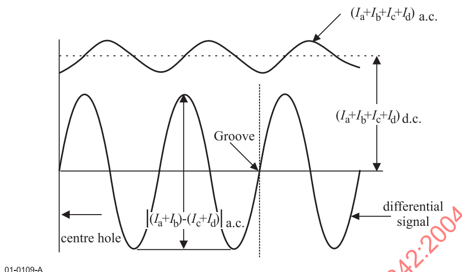
Figure 22 - Radial push-pull tracking error signal
