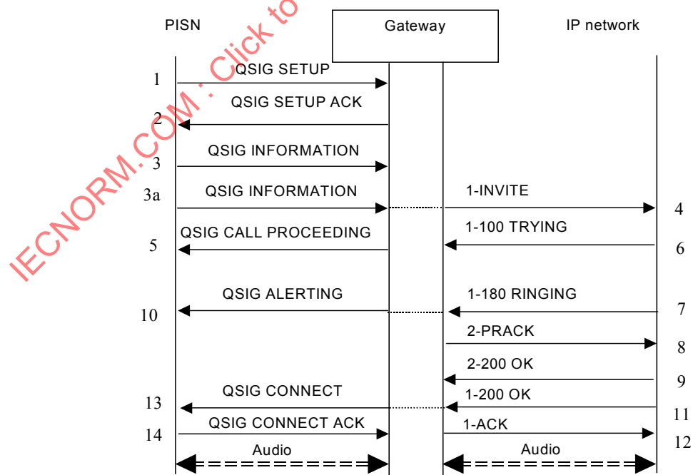
Figure 4 — Typical message sequence for successful call establishment from QSIG to SIP, using overlap receiving on QSIG and en bloc sending on SIP
