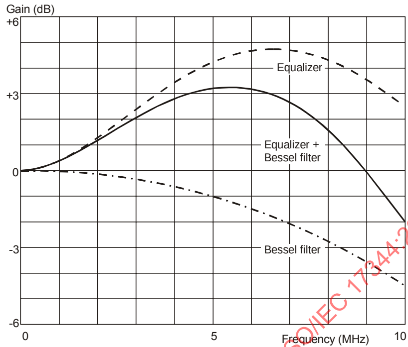
Figure D.3 - Frequency characteristics for the equalizer and the low-pass filter
