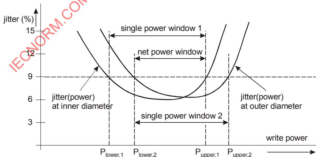
Figure 31 - Example of the write power windows
