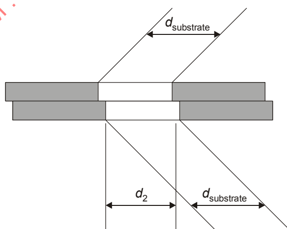
Figure 6 - Hole diameters for an assembled disk
