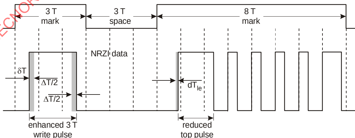
Figure F.2 - Example of a Multiple-pulse
