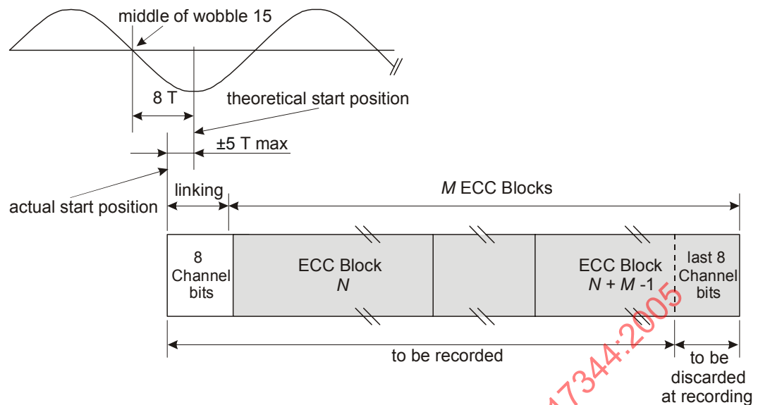
Figure 17 - Recording Unit
