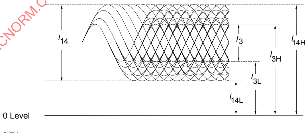
Figure 32 - Signals from spaces and marks in Read channel 1
