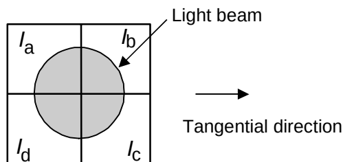
Figure 33 - Quadrant photo detector
