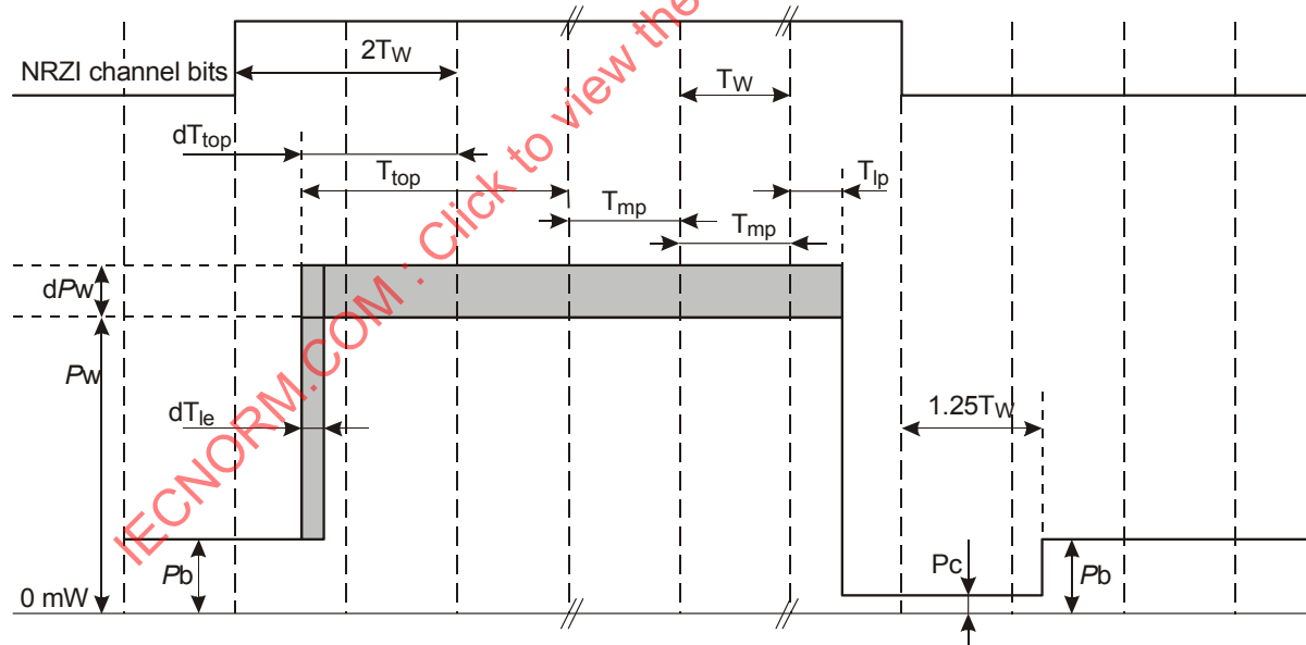
Figure F.3 – General blocked waveform
