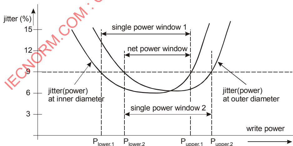
Figure 31 — Example of the write power windows
