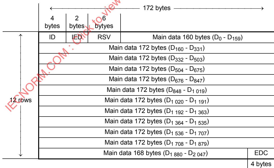
Figure 10 — Data Frame
