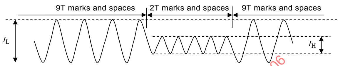
Figure 28 — Definition of I_L and I_H for resolution measurement
