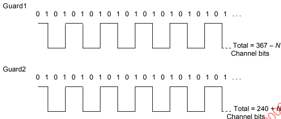
Figure 23 — Guard field patterns
