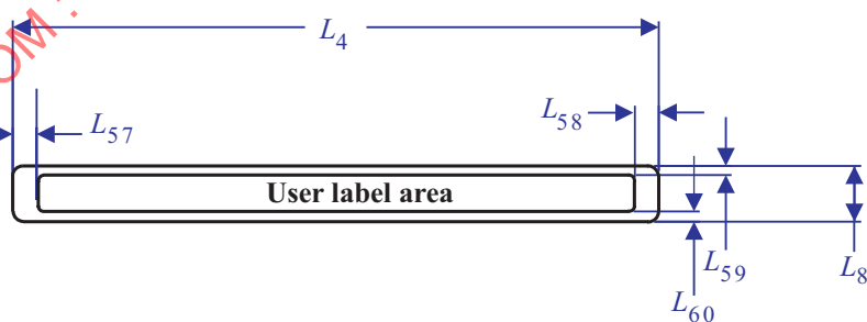
Figure 11b — User label area on bottom surface
