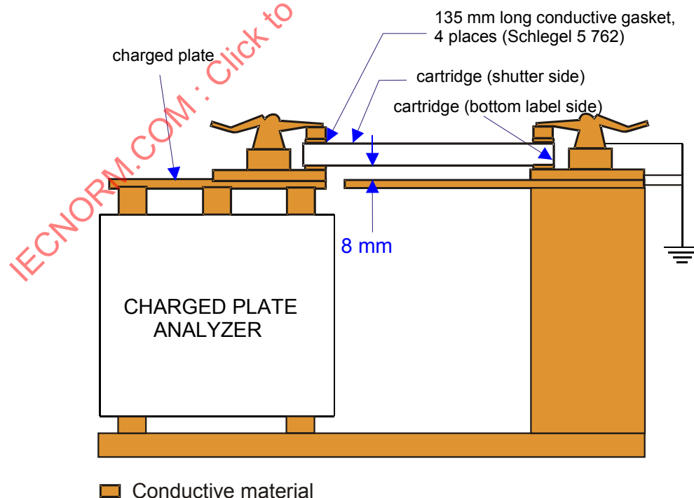
Figure D.1 — Cartridge electro-static discharge test fixture
