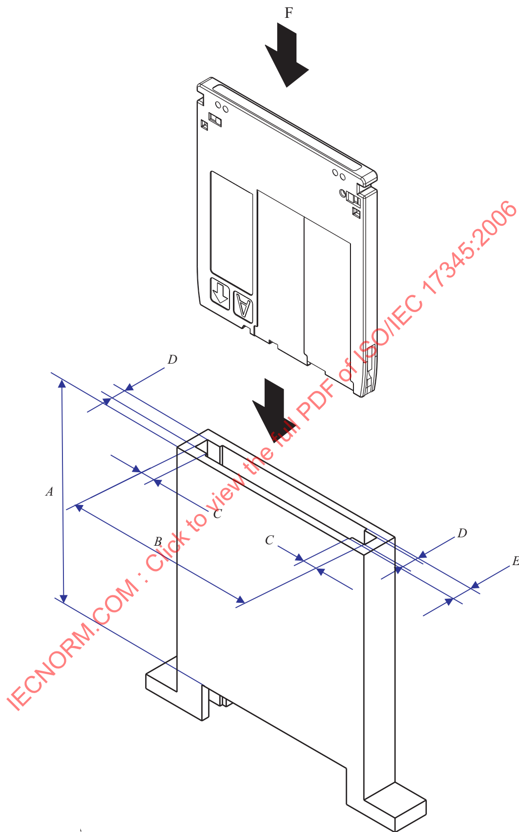
Figure B.1 — Distortion gauge
