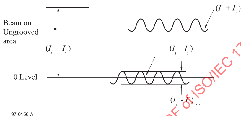
Figure 43 - Signals from lands and grooves in the Tracking channel
