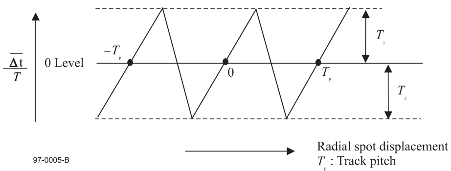
Figure 53 - Differential phase tracking error signal
