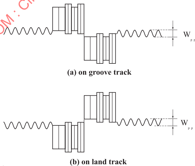
Figure 50 - Schematic representation of the signals from a groove or a land in Read channel 2
