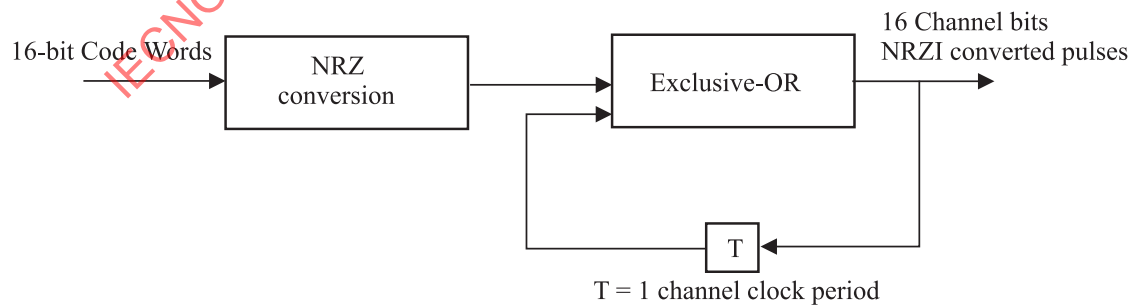
Figure 15 - NRZI conversion
