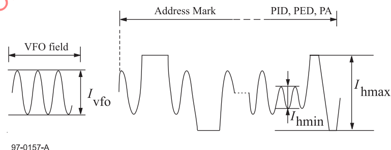
Figure 44b - Signals from Header field in Read channel 2
