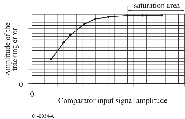
Figure C.2 - Comparator input signal amplitude vs tracking error signal amplitude
