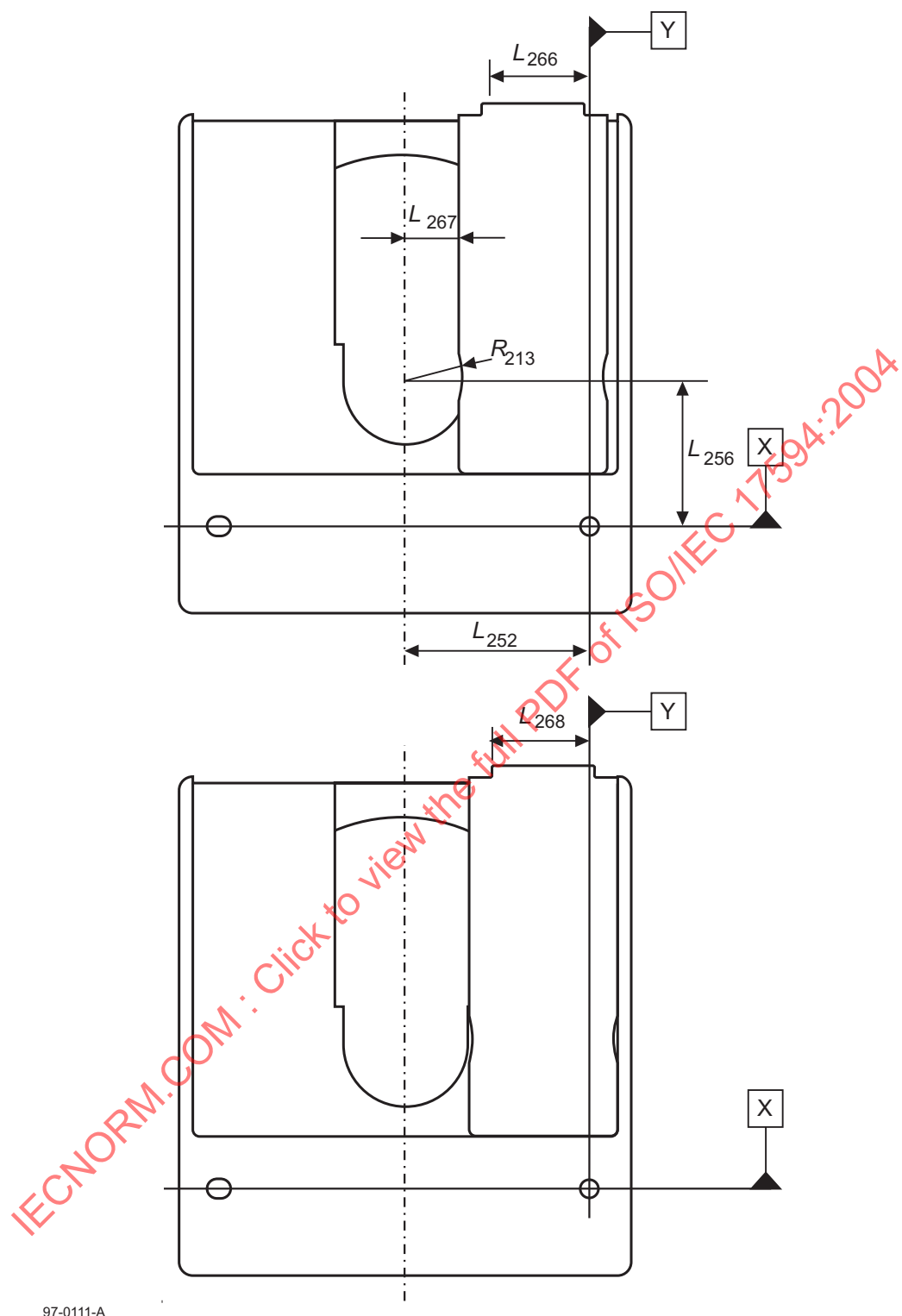
Figure 22 - Shutter in just right-hand open position (top view) and maximum right-hand open position (bottom view)
