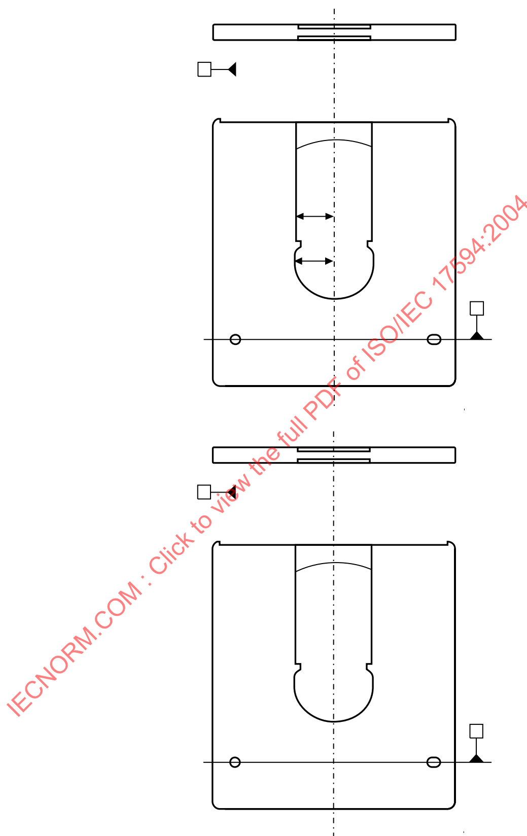
Figure 34 - Shutter in just open position (top view) and maximum open position (bottom view)
